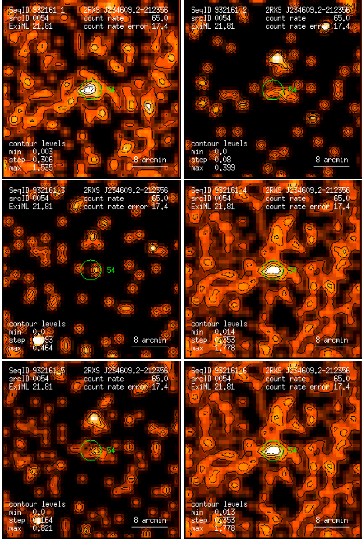
Figure 54: RASS 932161: detection 0054: band rate images, Gaussian filter: (1) PSPC channels 11 – 41, (2) 52 – 90, (3) 91 – 201, (4) 11 – 235, (5) 52 – 201, (6) 11 – 201. Broad band rates in counts/ks. Band rate contour levels in counts/ks/arcmin 2 .
