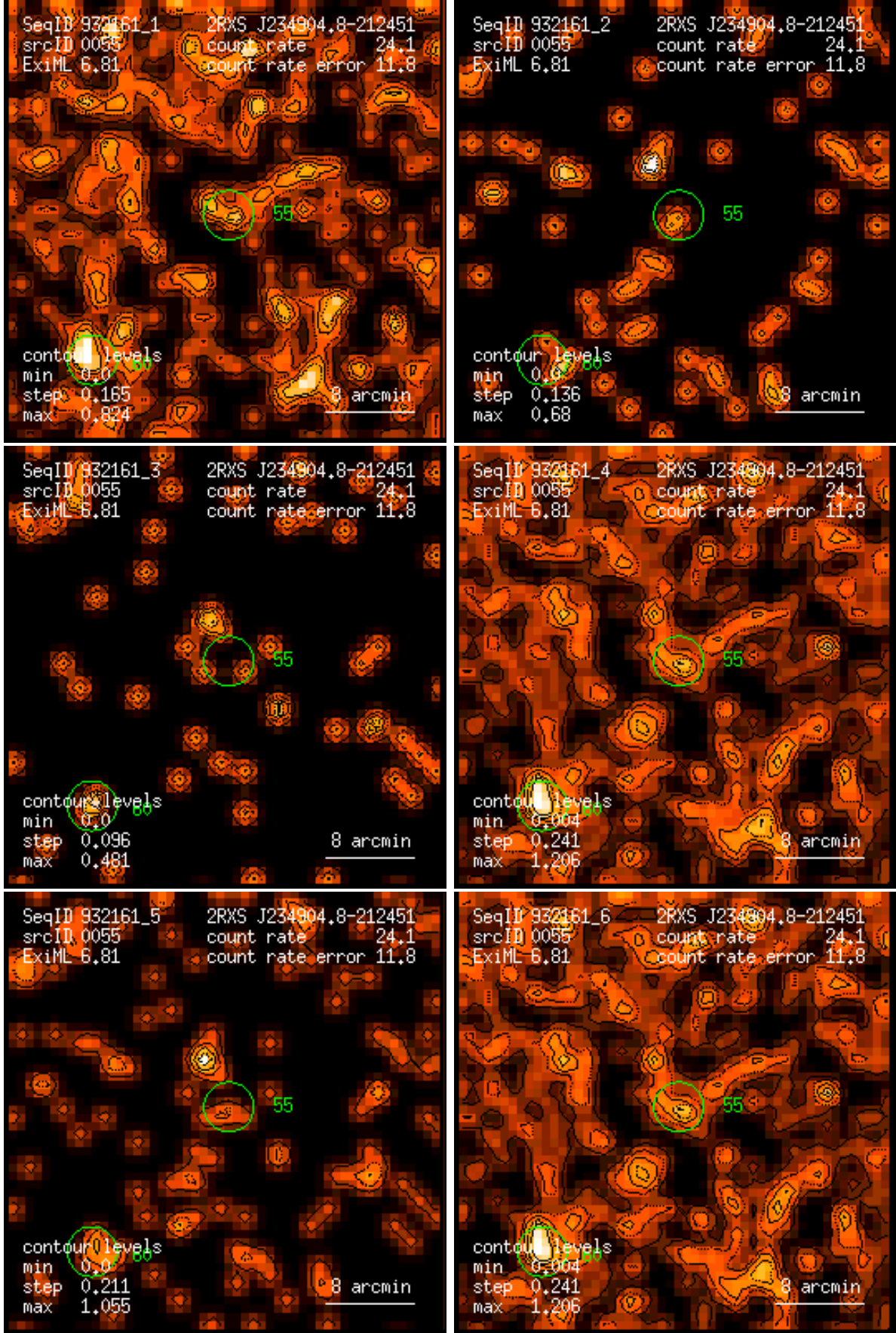
Figure 55: RASS 932161: detection 0055: band rate images, Gaussian filter: (1) PSPC channels 11 – 41, (2) 52 – 90, (3) 91 – 201, (4) 11 – 235, (5) 52 – 201, (6) 11 – 201. Broad band rates in counts/ks. Band rate contour levels in counts/ks/arcmin 2 .
