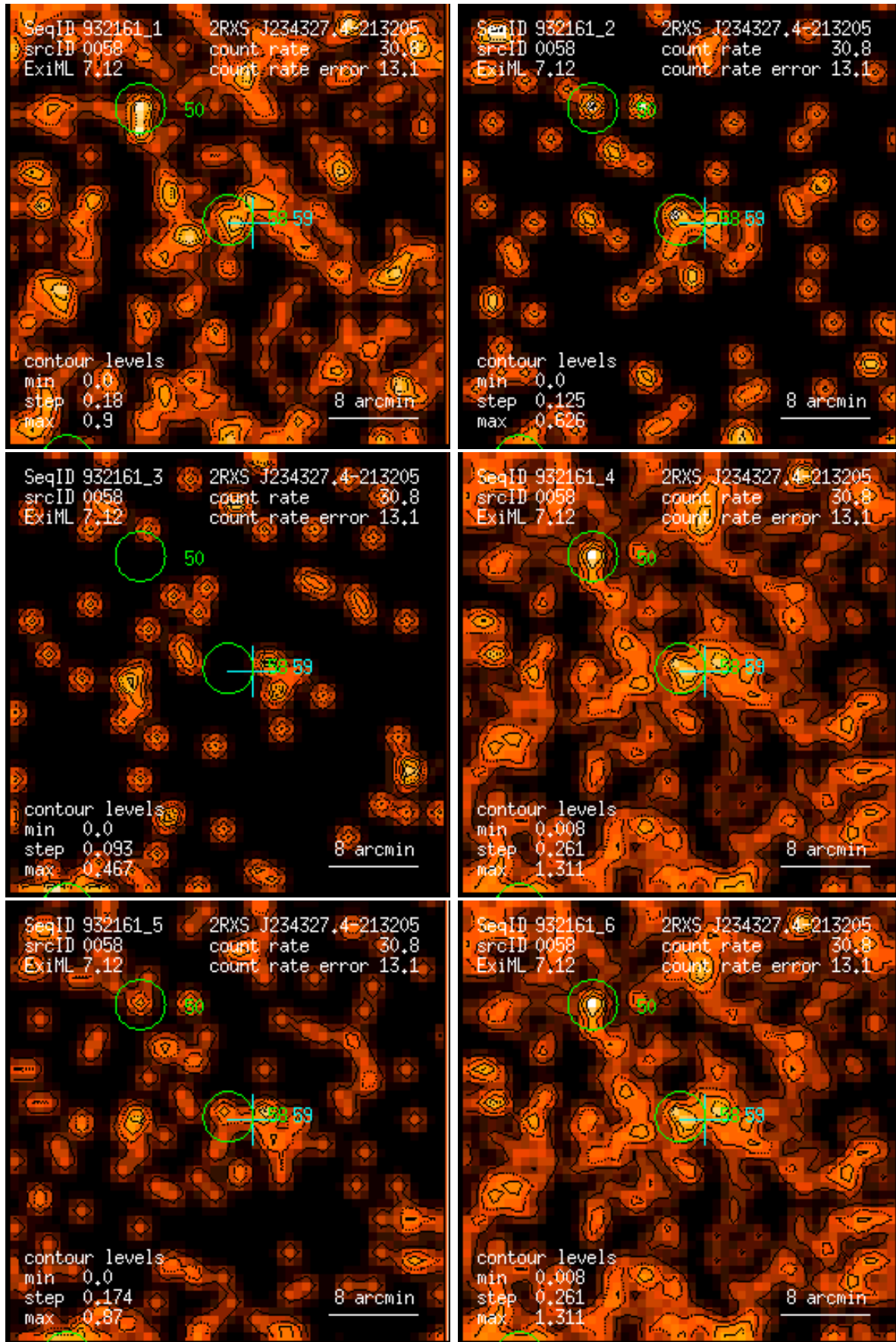
Figure 58: RASS 932161: detection 0058: band rate images, Gaussian filter: (1) PSPC channels 11 – 41, (2) 52 – 90, (3) 91 – 201, (4) 11 – 235, (5) 52 – 201, (6) 11 – 201. Broad band rates in counts/ks. Band rate contour levels in counts/ks/arcmin 2 .
