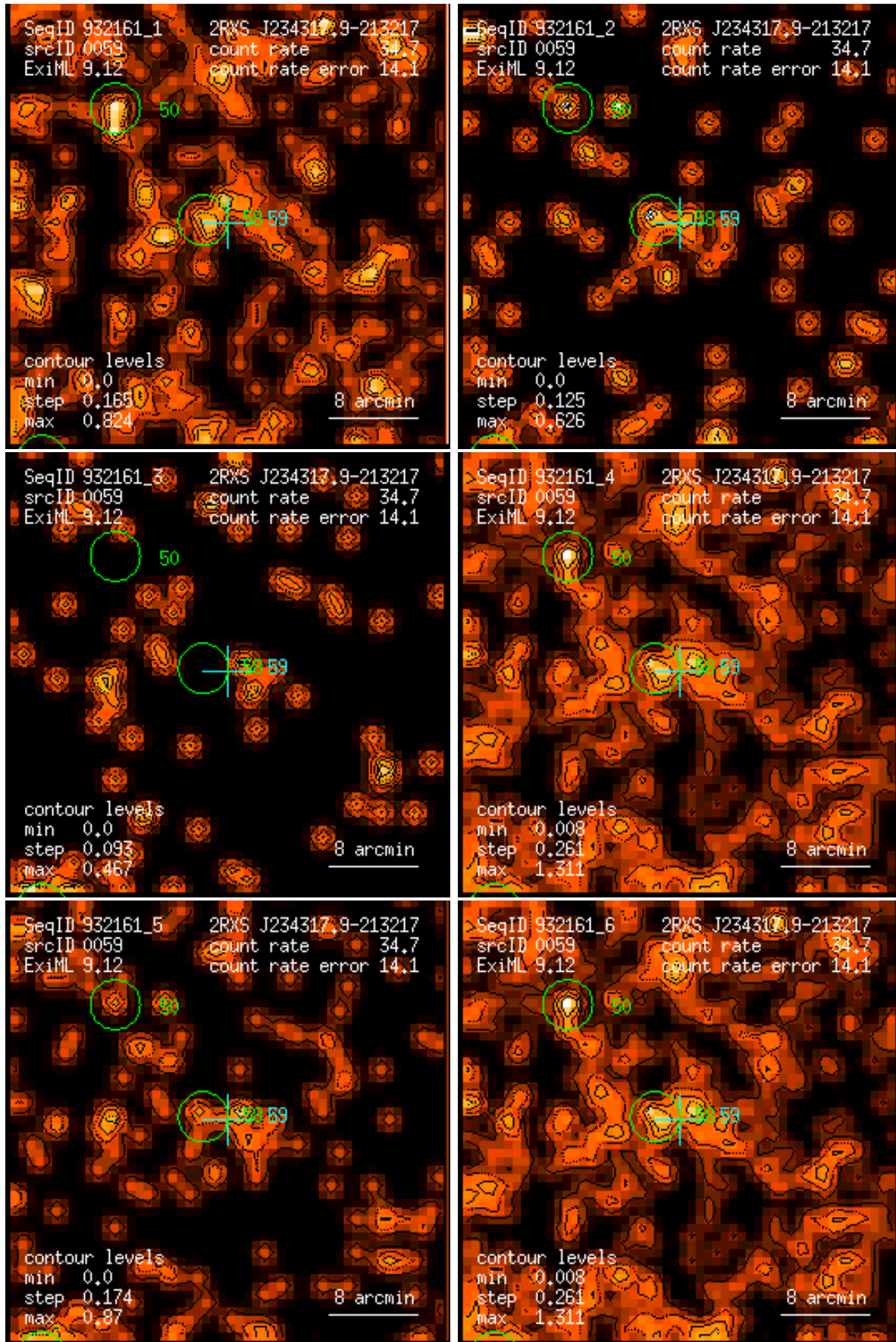
Figure 59: RASS 932161: detection 0059: band rate images, Gaussian filter: (1) PSPC channels 11 – 41, (2) 52 – 90, (3) 91 – 201, (4) 11 – 235, (5) 52 – 201, (6) 11 – 201. Broad band rates in counts/ks. Band rate contour levels in counts/ks/arcmin 2 .
