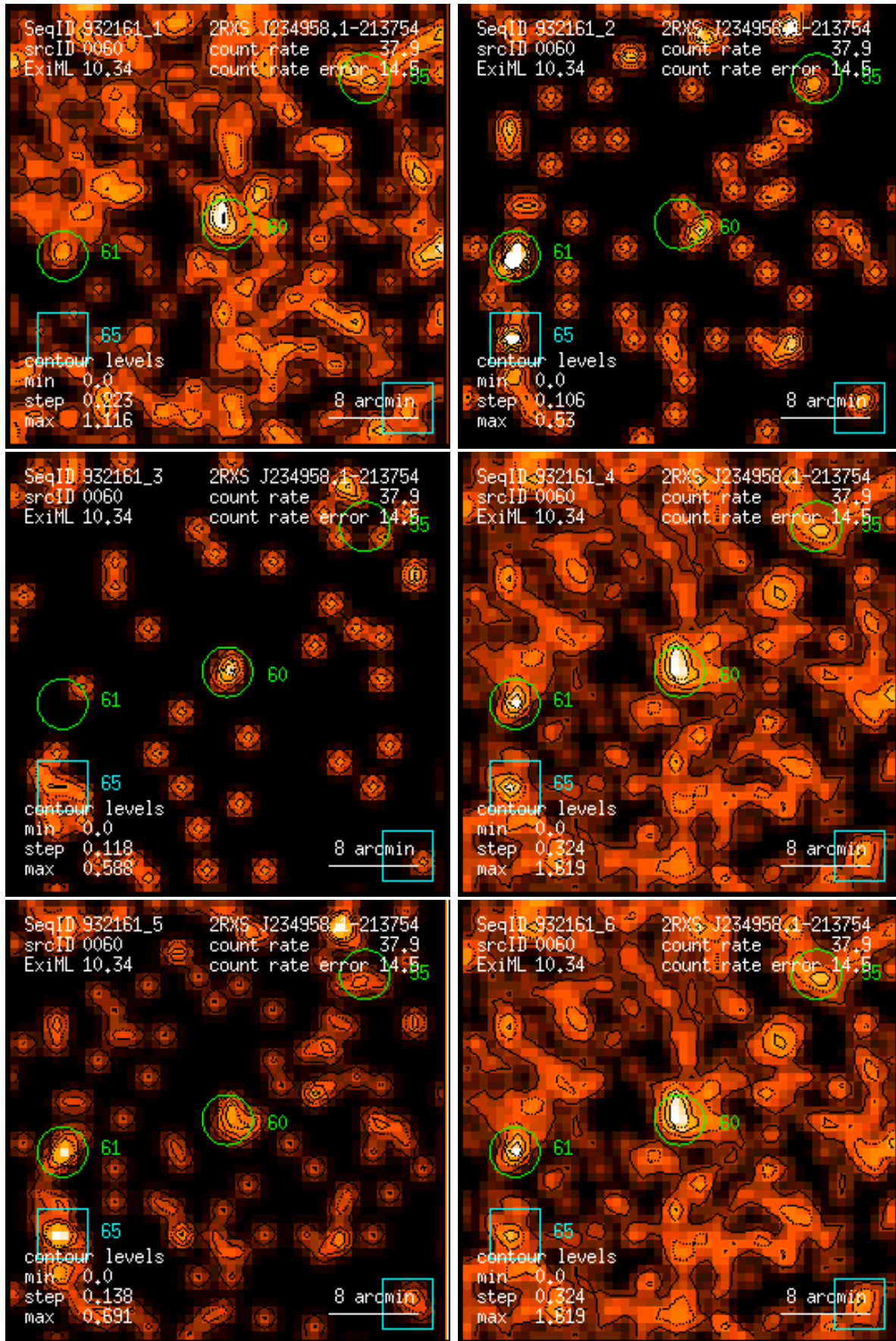
Figure 60: RASS 932161: detection 0060: band rate images, Gaussian filter: (1) PSPC channels 11 – 41, (2) 52 – 90, (3) 91 – 201, (4) 11 – 235, (5) 52 – 201, (6) 11 – 201. Broad band rates in counts/ks. Band rate contour levels in counts/ks/arcmin 2 .
