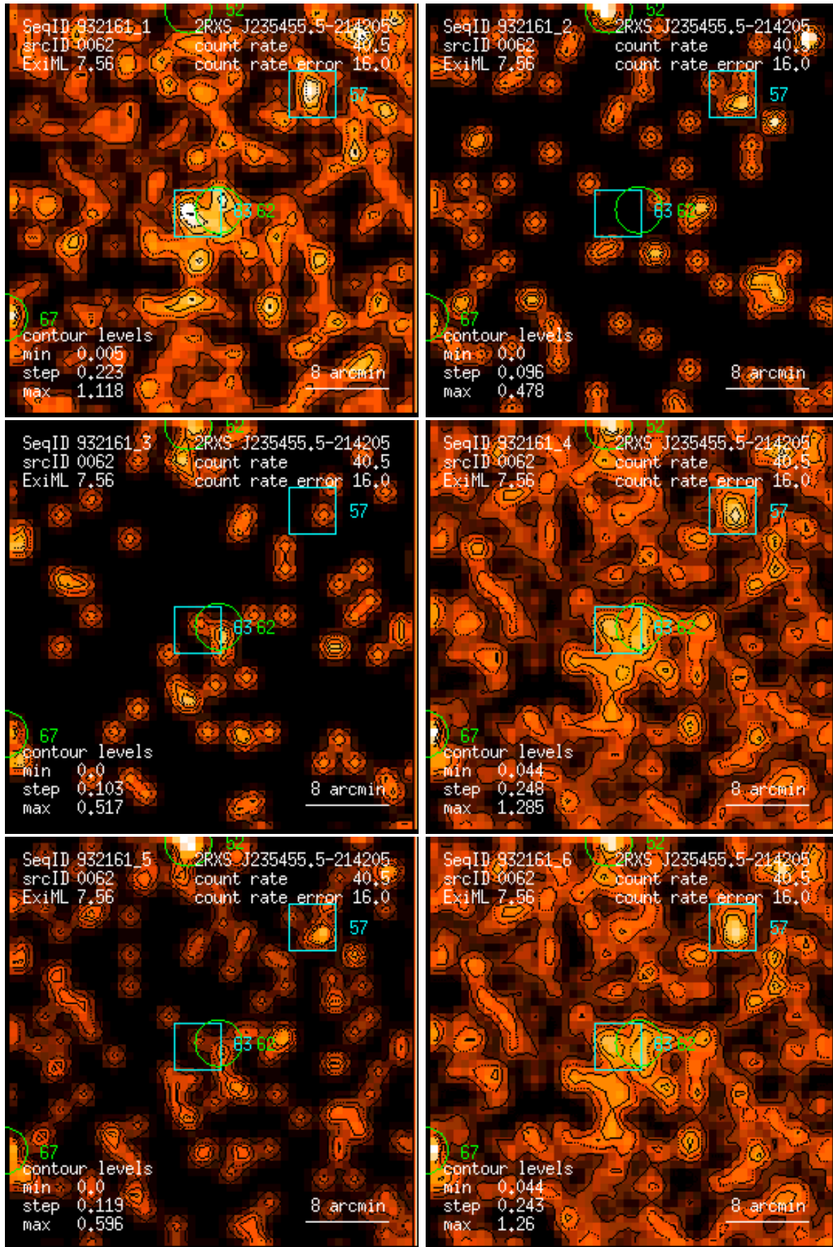
Figure 62: RASS 932161: detection 0062: band rate images, Gaussian filter: (1) PSPC channels 11 – 41, (2) 52 – 90, (3) 91 – 201, (4) 11 – 235, (5) 52 – 201, (6) 11 – 201. Broad band rates in counts/ks. Band rate contour levels in counts/ks/arcmin 2 .
