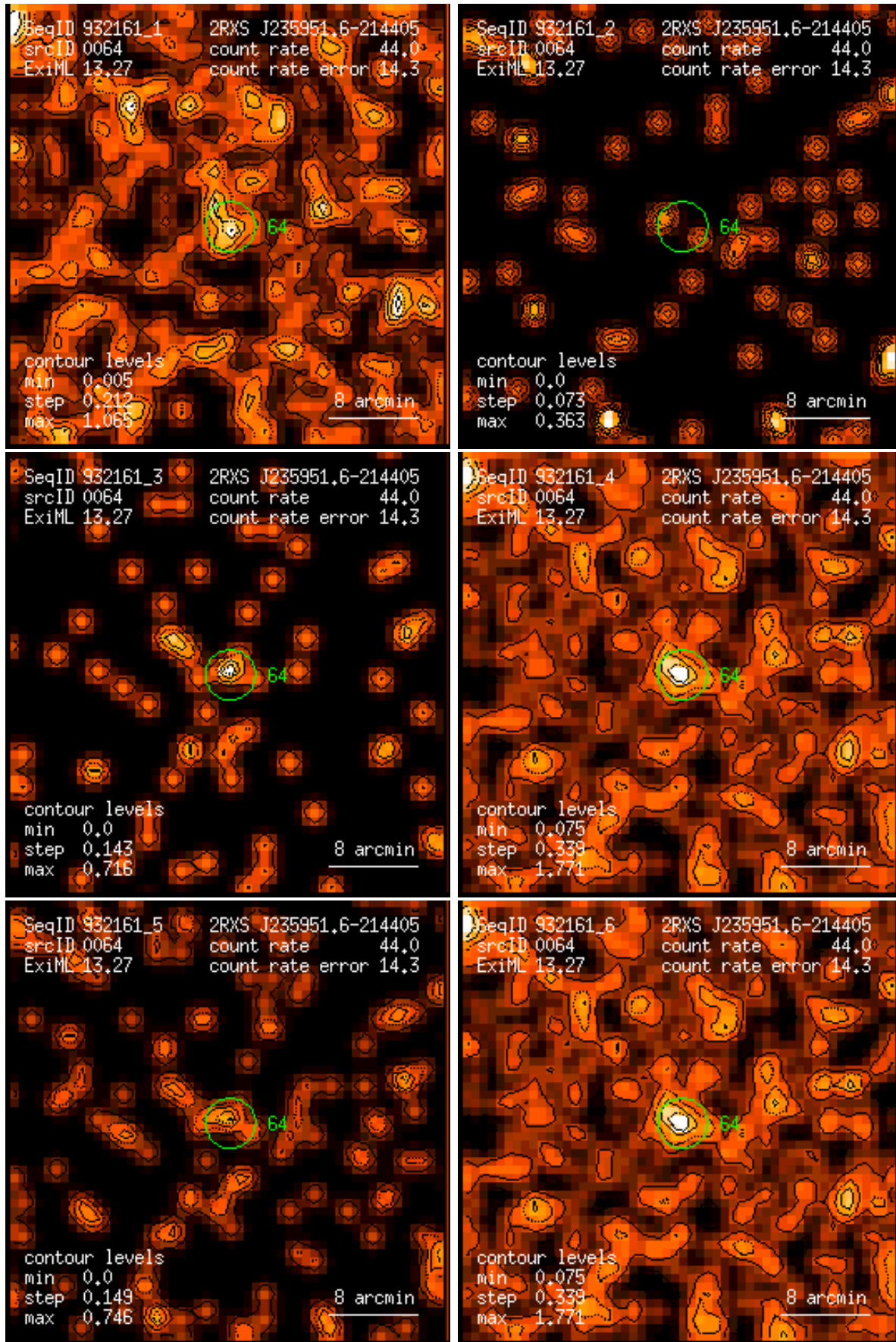
Figure 64: RASS 932161: detection 0064: band rate images, Gaussian filter: (1) PSPC channels 11 – 41, (2) 52 – 90, (3) 91 – 201, (4) 11 – 235, (5) 52 – 201, (6) 11 – 201. Broad band rates in counts/ks. Band rate contour levels in counts/ks/arcmin 2 .
