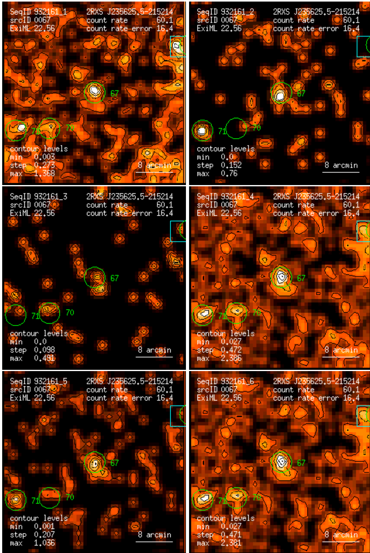
Figure 67: RASS 932161: detection 0067: band rate images, Gaussian filter: (1) PSPC channels 11 – 41, (2) 52 – 90, (3) 91 – 201, (4) 11 – 235, (5) 52 – 201, (6) 11 – 201. Broad band rates in counts/ks. Band rate contour levels in counts/ks/arcmin 2 .
