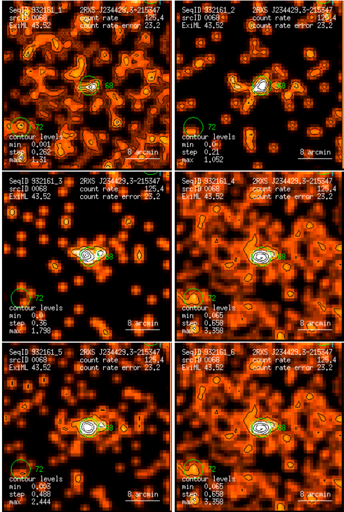
Figure 68: RASS 932161: detection 0068: band rate images, Gaussian filter: (1) PSPC channels 11 – 41, (2) 52 – 90, (3) 91 – 201, (4) 11 – 235, (5) 52 – 201, (6) 11 – 201. Broad band rates in counts/ks. Band rate contour levels in counts/ks/arcmin 2 .
