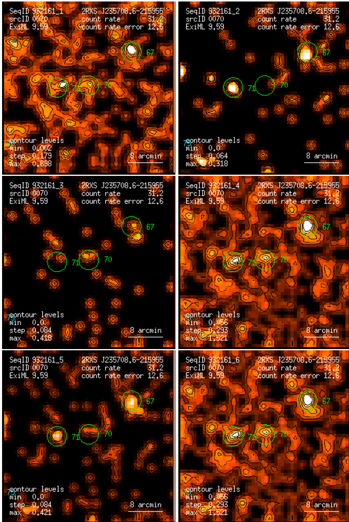
Figure 70: RASS 932161: detection 0070: band rate images, Gaussian filter: (1) PSPC channels 11 – 41, (2) 52 – 90, (3) 91 – 201, (4) 11 – 235, (5) 52 – 201, (6) 11 – 201. Broad band rates in counts/ks. Band rate contour levels in counts/ks/arcmin 2 .
