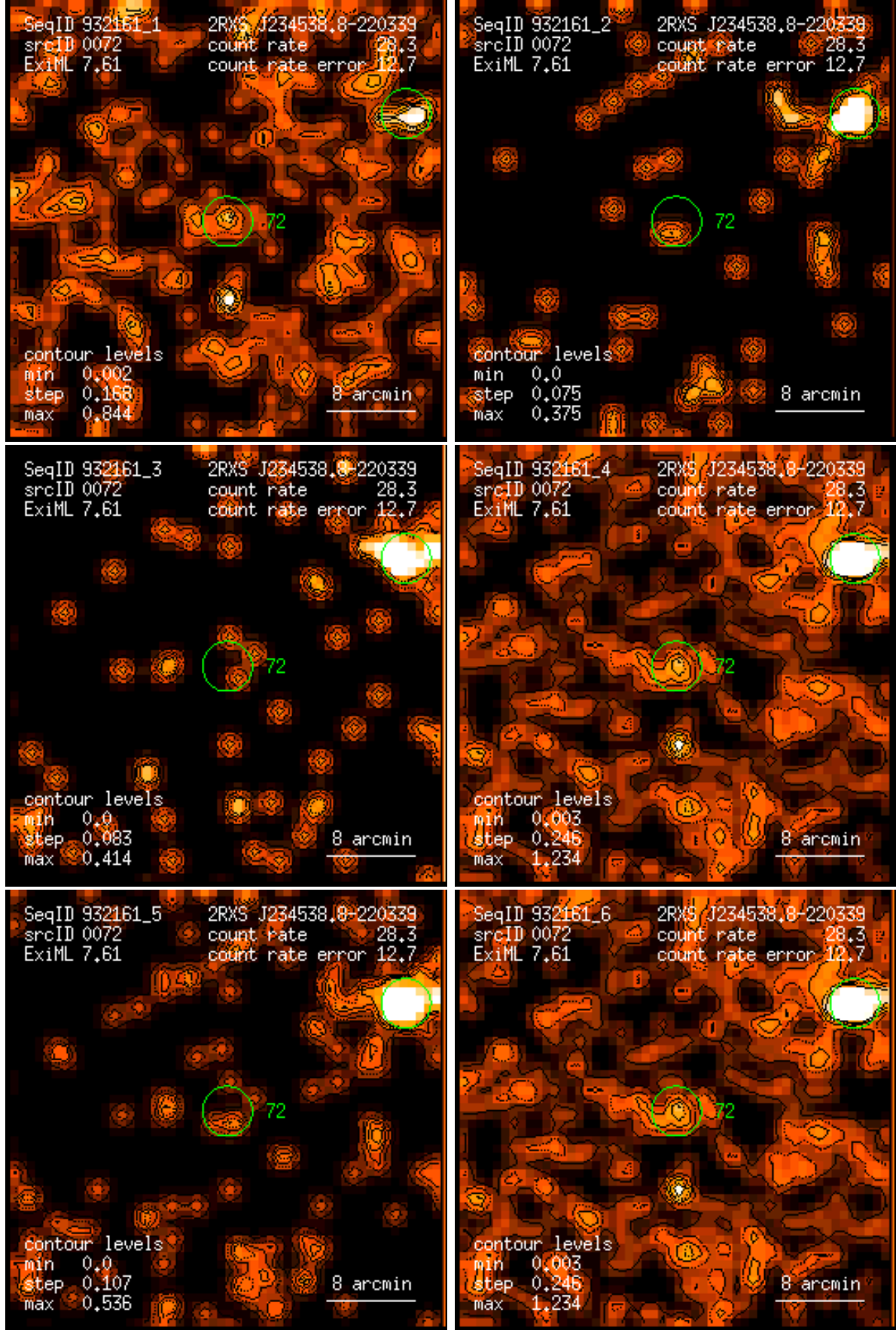
Figure 72: RASS 932161: detection 0072: band rate images, Gaussian filter: (1) PSPC channels 11 – 41, (2) 52 – 90, (3) 91 – 201, (4) 11 – 235, (5) 52 – 201, (6) 11 – 201. Broad band rates in counts/ks. Band rate contour levels in counts/ks/arcmin 2 .
