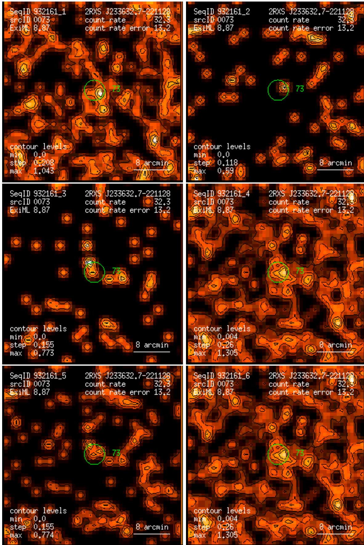
Figure 73: RASS 932161: detection 0073: band rate images, Gaussian filter: (1) PSPC channels 11 – 41, (2) 52 – 90, (3) 91 – 201, (4) 11 – 235, (5) 52 – 201, (6) 11 – 201. Broad band rates in counts/ks. Band rate contour levels in counts/ks/arcmin 2 .
