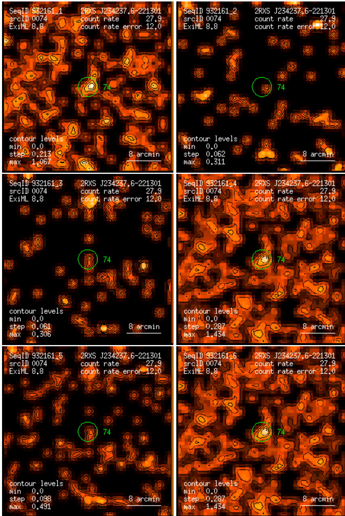
Figure 74: RASS 932161: detection 0074: band rate images, Gaussian filter: (1) PSPC channels 11 – 41, (2) 52 – 90, (3) 91 – 201, (4) 11 – 235, (5) 52 – 201, (6) 11 – 201. Broad band rates in counts/ks. Band rate contour levels in counts/ks/arcmin 2 .
