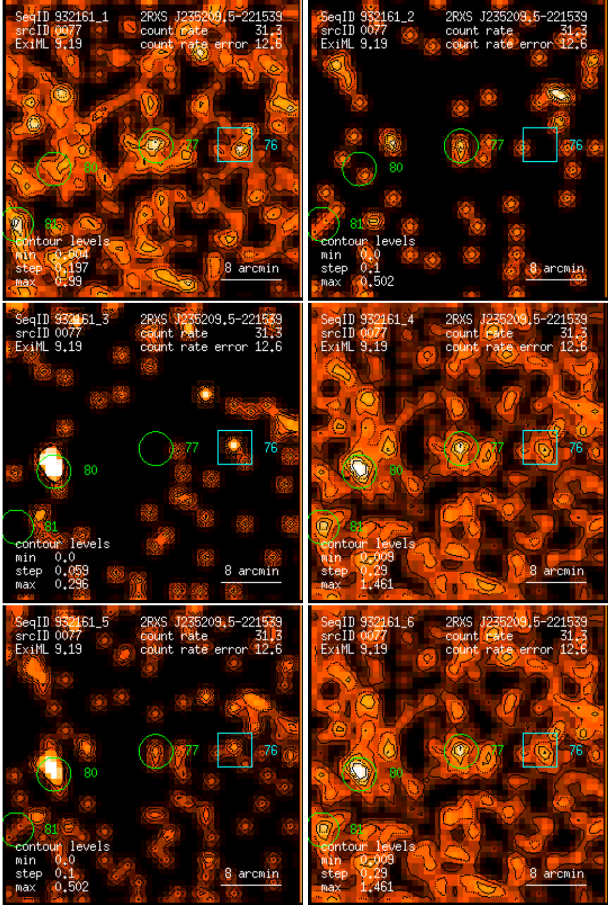
Figure 77: RASS 932161: detection 0077: band rate images, Gaussian filter: (1) PSPC channels 11 – 41, (2) 52 – 90, (3) 91 – 201, (4) 11 – 235, (5) 52 – 201, (6) 11 – 201. Broad band rates in counts/ks. Band rate contour levels in counts/ks/arcmin 2 .
