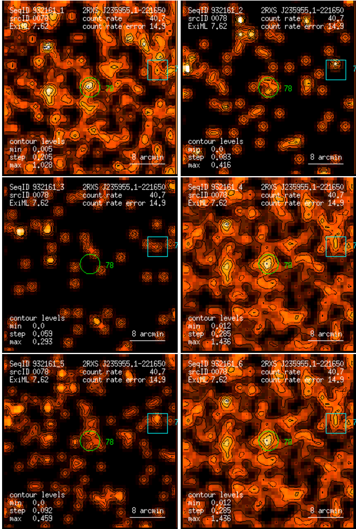
Figure 78: RASS 932161: detection 0078: band rate images, Gaussian filter: (1) PSPC channels 11 – 41, (2) 52 – 90, (3) 91 – 201, (4) 11 – 235, (5) 52 – 201, (6) 11 – 201. Broad band rates in counts/ks. Band rate contour levels in counts/ks/arcmin 2 .
