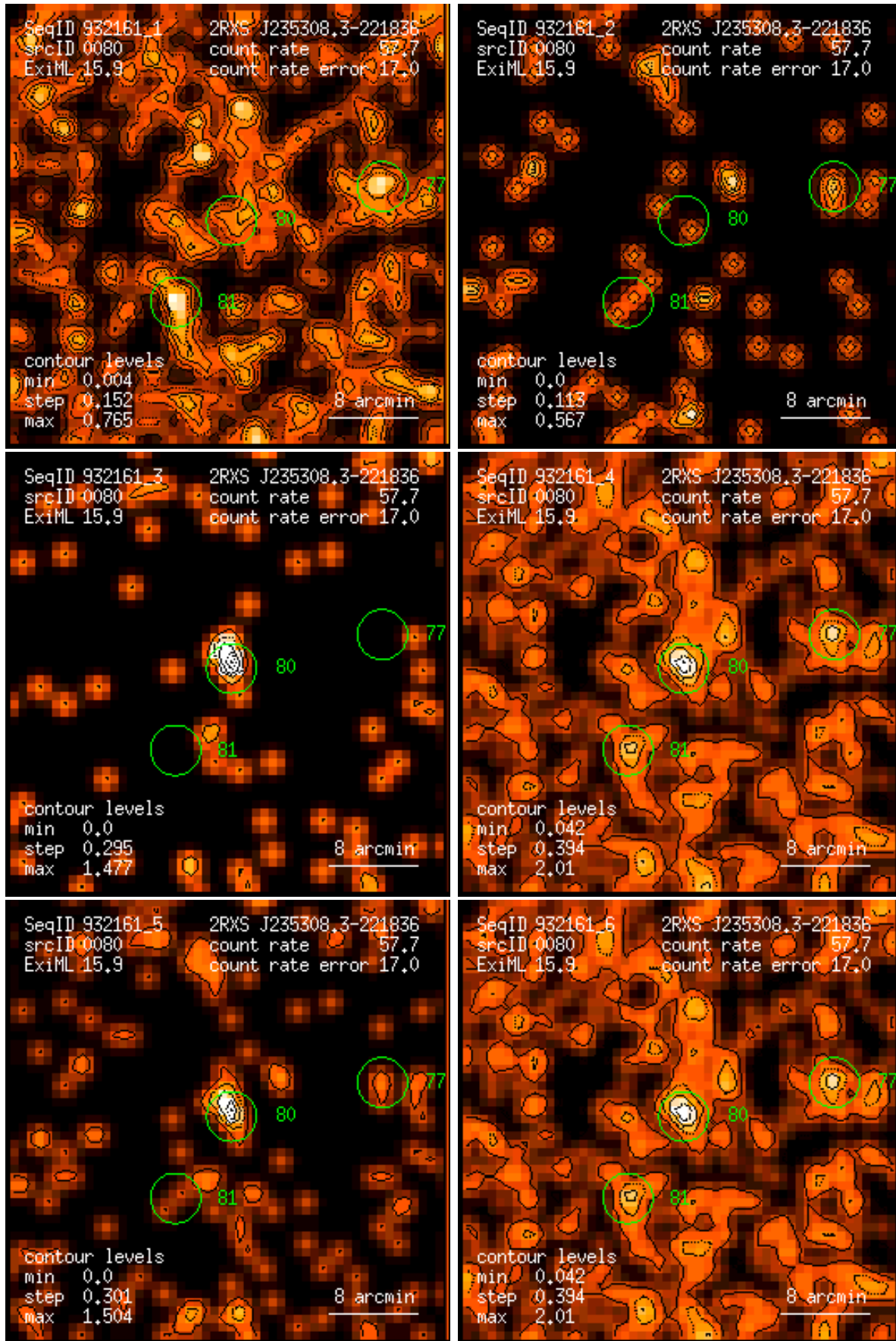
Figure 80: RASS 932161: detection 0080: band rate images, Gaussian filter: (1) PSPC channels 11 – 41, (2) 52 – 90, (3) 91 – 201, (4) 11 – 235, (5) 52 – 201, (6) 11 – 201. Broad band rates in counts/ks. Band rate contour levels in counts/ks/arcmin 2 .
