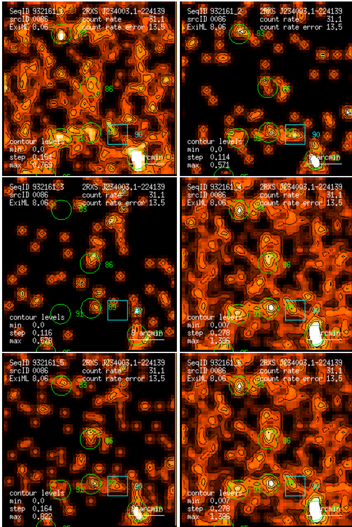
Figure 86: RASS 932161: detection 0086: band rate images, Gaussian filter: (1) PSPC channels 11 – 41, (2) 52 – 90, (3) 91 – 201, (4) 11 – 235, (5) 52 – 201, (6) 11 – 201. Broad band rates in counts/ks. Band rate contour levels in counts/ks/arcmin 2 .
