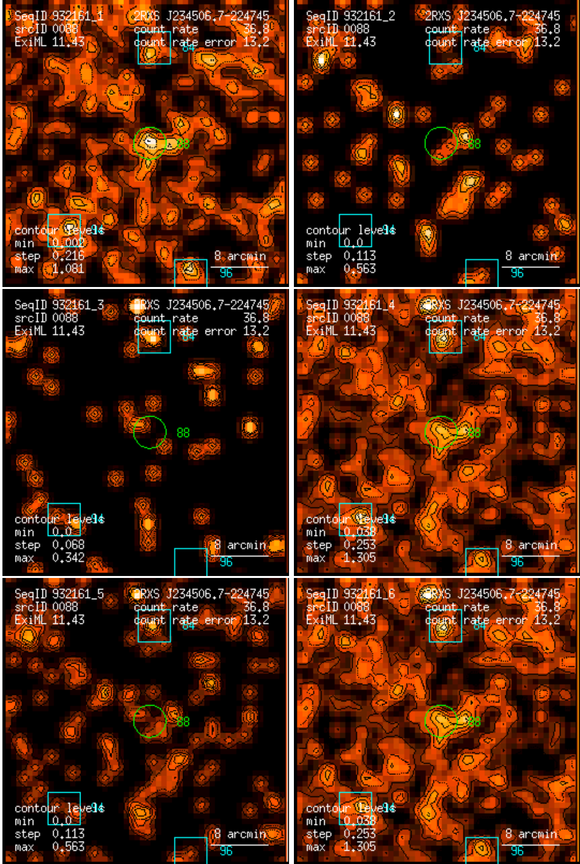
Figure 88: RASS 932161: detection 0088: band rate images, Gaussian filter: (1) PSPC channels 11 – 41, (2) 52 – 90, (3) 91 – 201, (4) 11 – 235, (5) 52 – 201, (6) 11 – 201. Broad band rates in counts/ks. Band rate contour levels in counts/ks/arcmin 2 .
