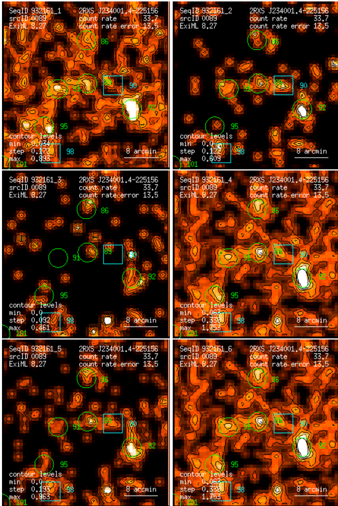
Figure 89: RASS 932161: detection 0089: band rate images, Gaussian filter: (1) PSPC channels 11 – 41, (2) 52 – 90, (3) 91 – 201, (4) 11 – 235, (5) 52 – 201, (6) 11 – 201. Broad band rates in counts/ks. Band rate contour levels in counts/ks/arcmin 2 .
