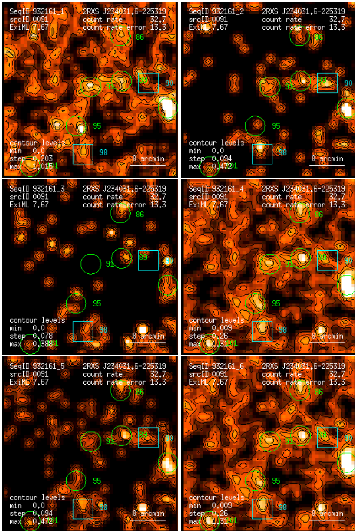
Figure 91: RASS 932161: detection 0091: band rate images, Gaussian filter: (1) PSPC channels 11 – 41, (2) 52 – 90, (3) 91 – 201, (4) 11 – 235, (5) 52 – 201, (6) 11 – 201. Broad band rates in counts/ks. Band rate contour levels in counts/ks/arcmin 2 .
