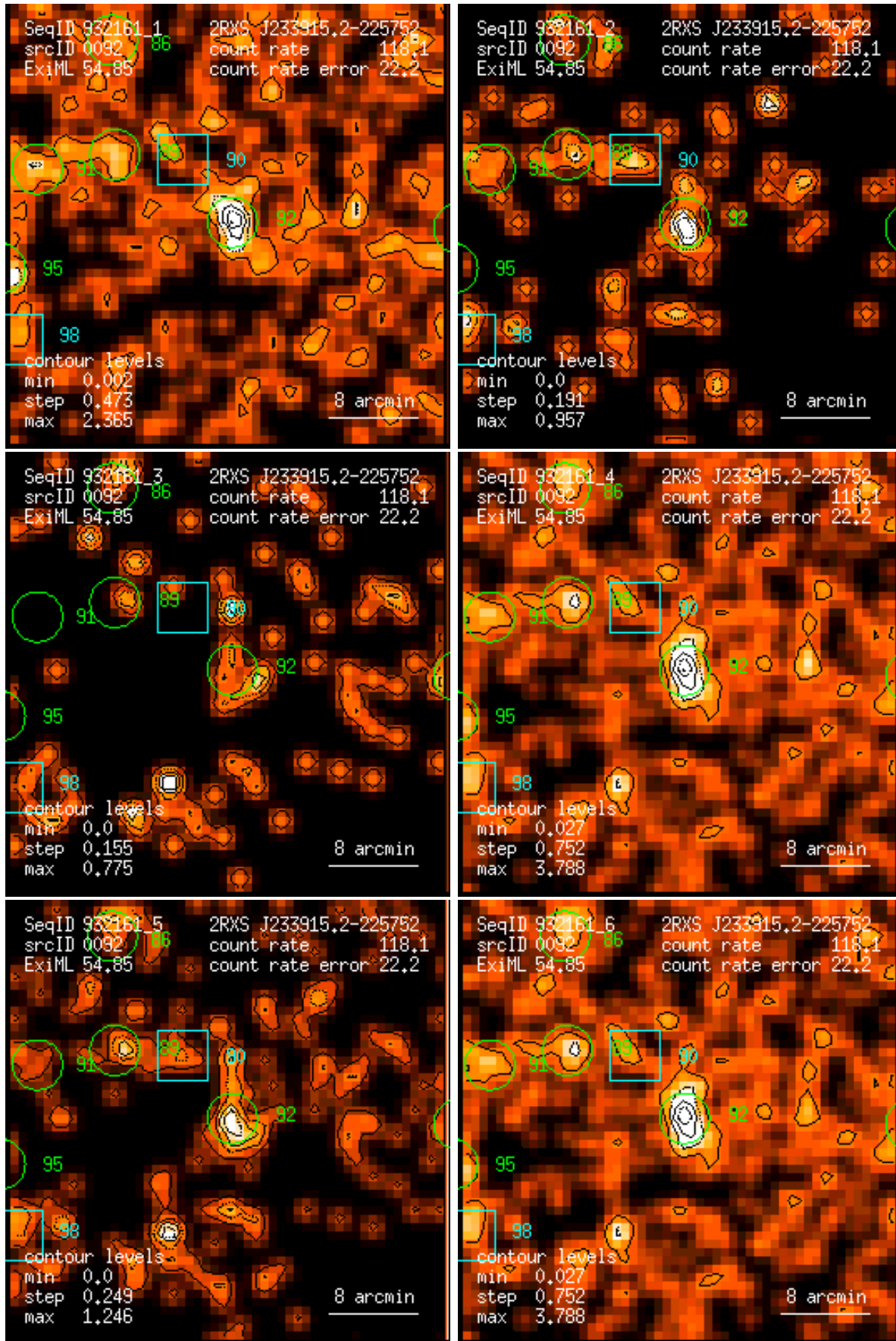
Figure 92: RASS 932161: detection 0092: band rate images, Gaussian filter: (1) PSPC channels 11 – 41, (2) 52 – 90, (3) 91 – 201, (4) 11 – 235, (5) 52 – 201, (6) 11 – 201. Broad band rates in counts/ks. Band rate contour levels in counts/ks/arcmin 2 .
