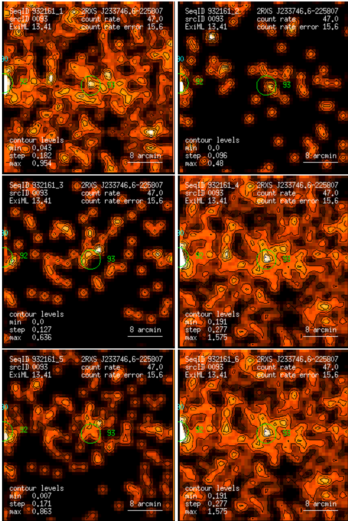
Figure 93: RASS 932161: detection 0093: band rate images, Gaussian filter: (1) PSPC channels 11 – 41, (2) 52 – 90, (3) 91 – 201, (4) 11 – 235, (5) 52 – 201, (6) 11 – 201. Broad band rates in counts/ks. Band rate contour levels in counts/ks/arcmin 2 .
