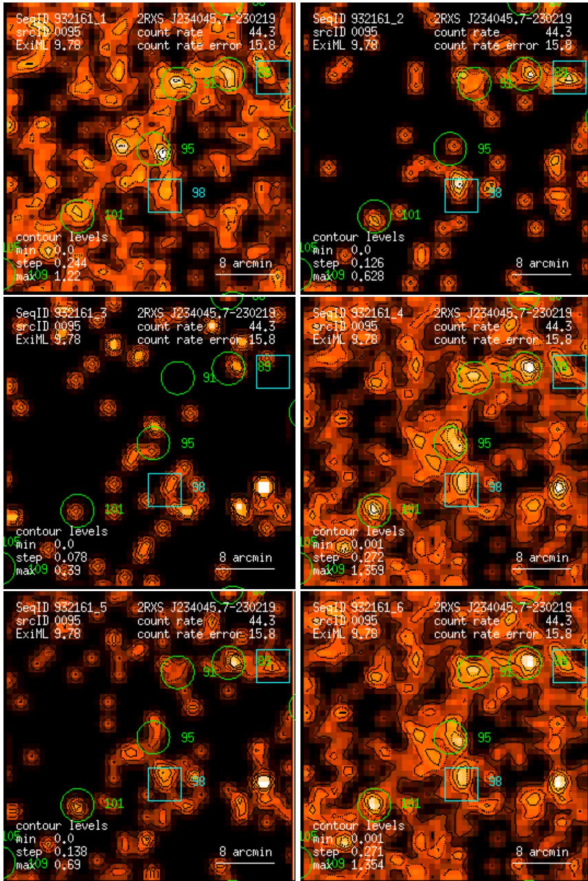
Figure 95: RASS 932161: detection 0095: band rate images, Gaussian filter: (1) PSPC channels 11 – 41, (2) 52 – 90, (3) 91 – 201, (4) 11 – 235, (5) 52 – 201, (6) 11 – 201. Broad band rates in counts/ks. Band rate contour levels in counts/ks/arcmin 2 .
