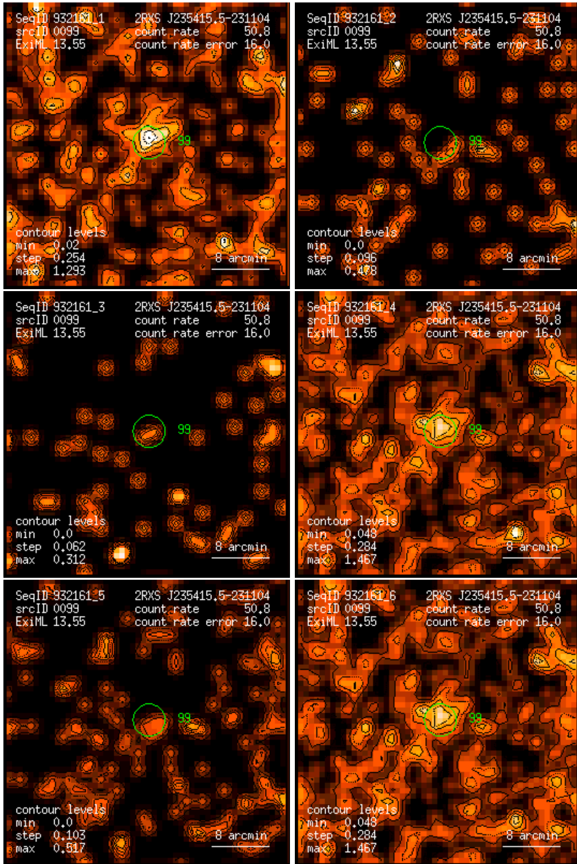
Figure 99: RASS 932161: detection 0099: band rate images, Gaussian filter: (1) PSPC channels 11 – 41, (2) 52 – 90, (3) 91 – 201, (4) 11 – 235, (5) 52 – 201, (6) 11 – 201. Broad band rates in counts/ks. Band rate contour levels in counts/ks/arcmin 2 .
