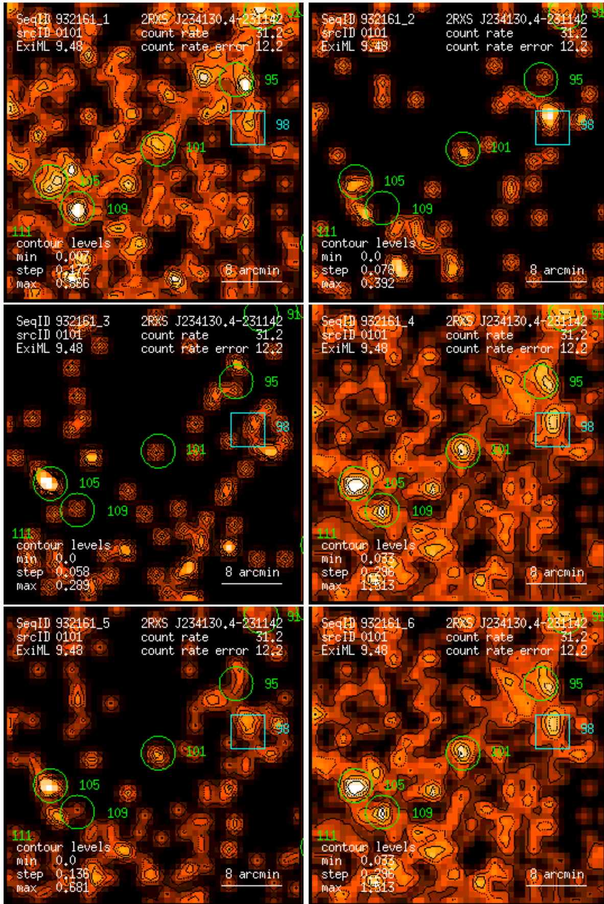
Figure 101: RASS 932161: detection 0101: band rate images, Gaussian filter: (1) PSPC channels 11 – 41, (2) 52 – 90, (3) 91 – 201, (4) 11 – 235, (5) 52 – 201, (6) 11 – 201. Broad band rates in counts/ks. Band rate contour levels in counts/ks/arcmin 2 .
