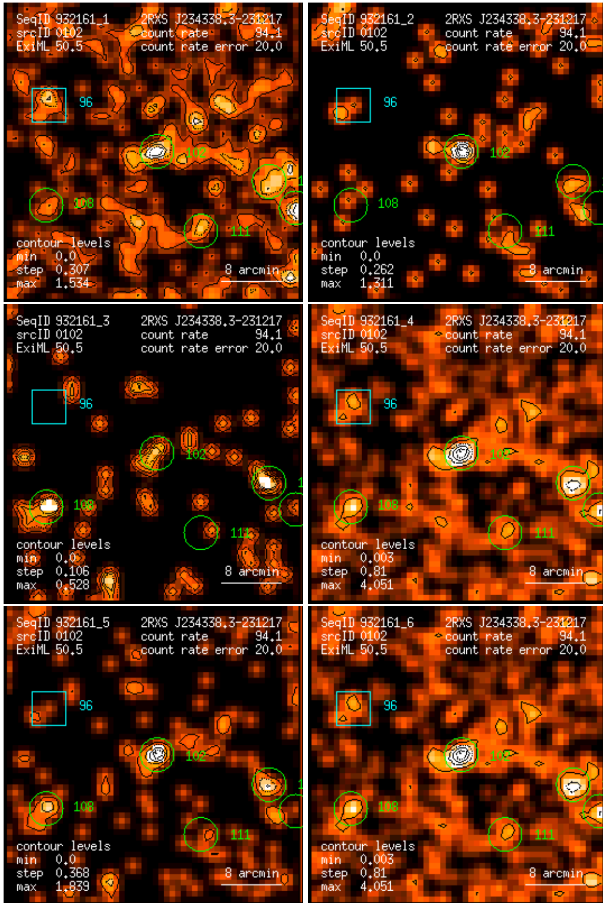
Figure 102: RASS 932161: detection 0102: band rate images, Gaussian filter: (1) PSPC channels 11 – 41, (2) 52 – 90, (3) 91 – 201, (4) 11 – 235, (5) 52 – 201, (6) 11 – 201. Broad band rates in counts/ks. Band rate contour levels in counts/ks/arcmin 2 .
