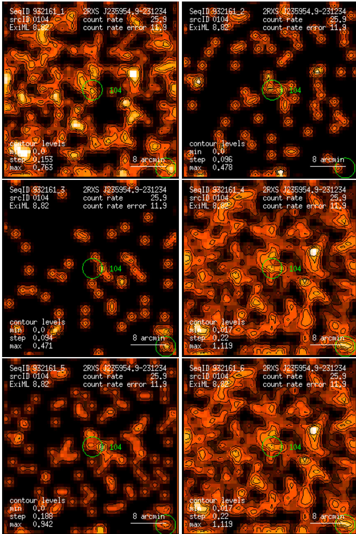
Figure 104: RASS 932161: detection 0104: band rate images, Gaussian filter: (1) PSPC channels 11 – 41, (2) 52 – 90, (3) 91 – 201, (4) 11 – 235, (5) 52 – 201, (6) 11 – 201. Broad band rates in counts/ks. Band rate contour levels in counts/ks/arcmin 2 .
