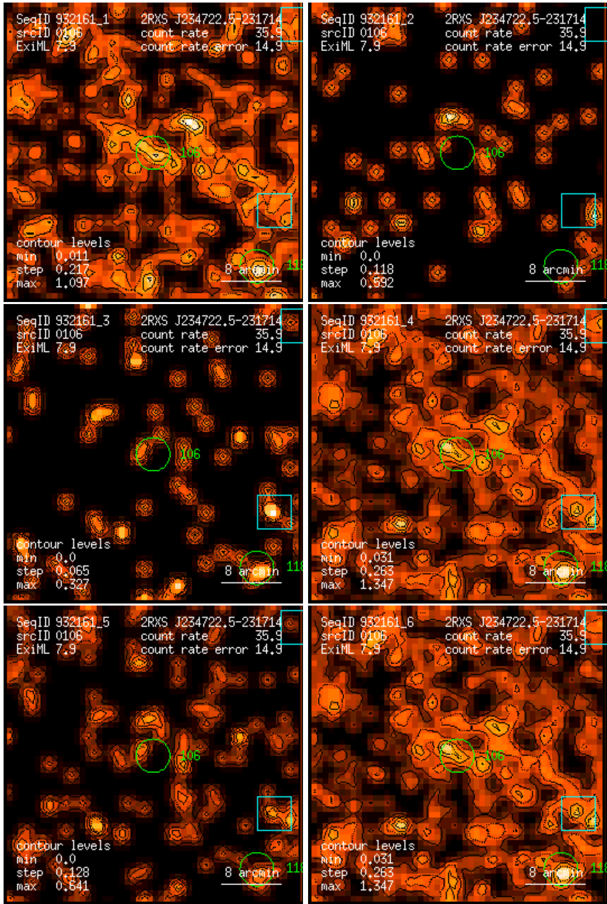
Figure 106: RASS 932161: detection 0106: band rate images, Gaussian filter: (1) PSPC channels 11 – 41, (2) 52 – 90, (3) 91 – 201, (4) 11 – 235, (5) 52 – 201, (6) 11 – 201. Broad band rates in counts/ks. Band rate contour levels in counts/ks/arcmin 2 .
