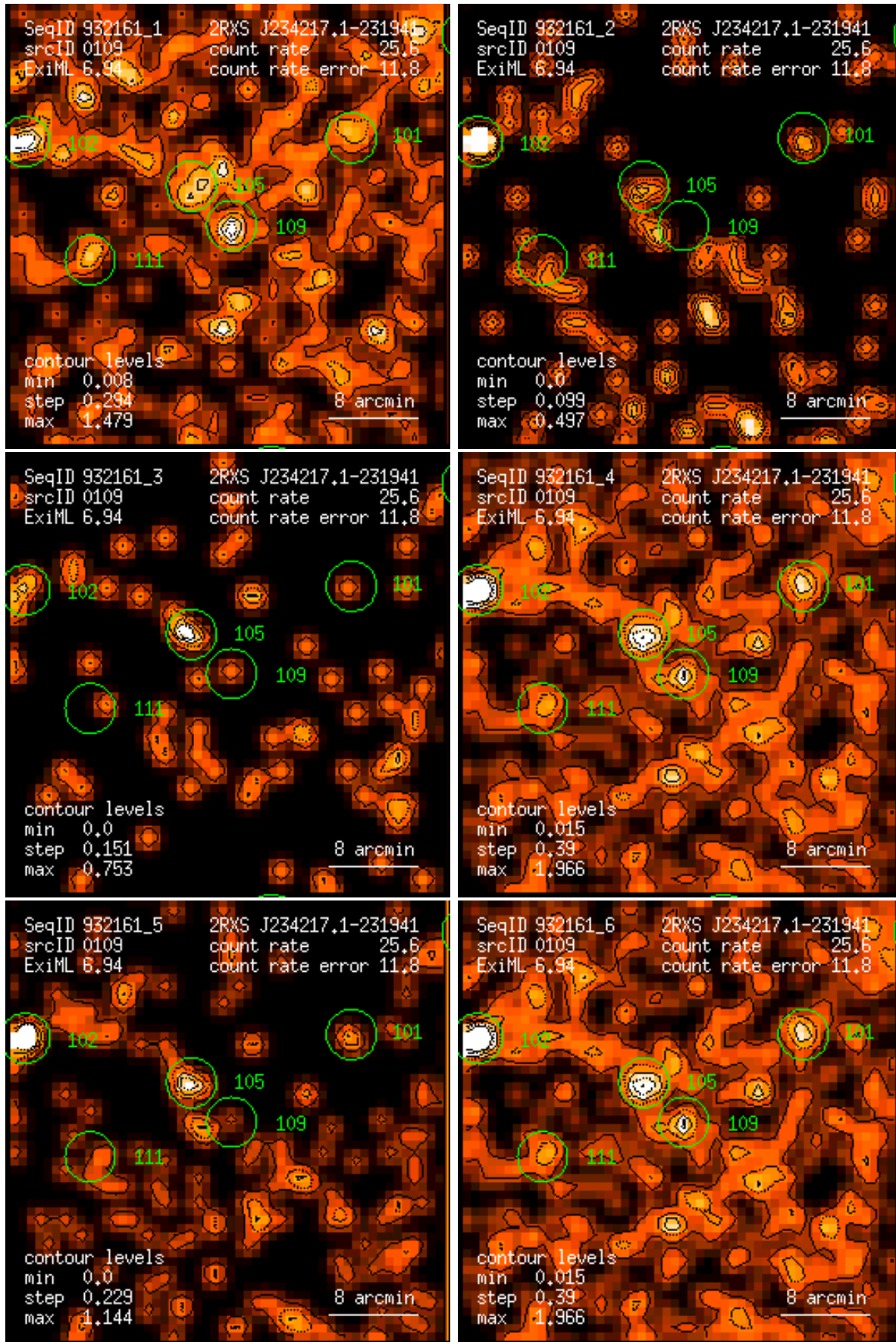
Figure 109: RASS 932161: detection 0109: band rate images, Gaussian filter: (1) PSPC channels 11 – 41, (2) 52 – 90, (3) 91 – 201, (4) 11 – 235, (5) 52 – 201, (6) 11 – 201. Broad band rates in counts/ks. Band rate contour levels in counts/ks/arcmin 2 .
