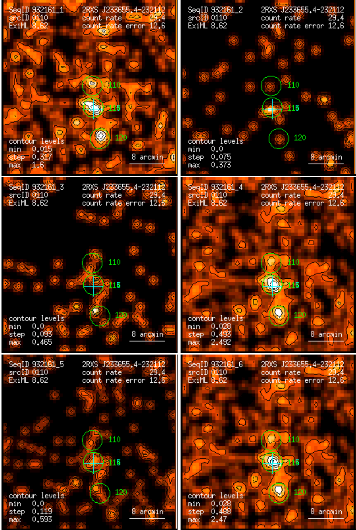
Figure 110: RASS 932161: detection 0110: band rate images, Gaussian filter: (1) PSPC channels 11 – 41, (2) 52 – 90, (3) 91 – 201, (4) 11 – 235, (5) 52 – 201, (6) 11 – 201. Broad band rates in counts/ks. Band rate contour levels in counts/ks/arcmin 2 .
