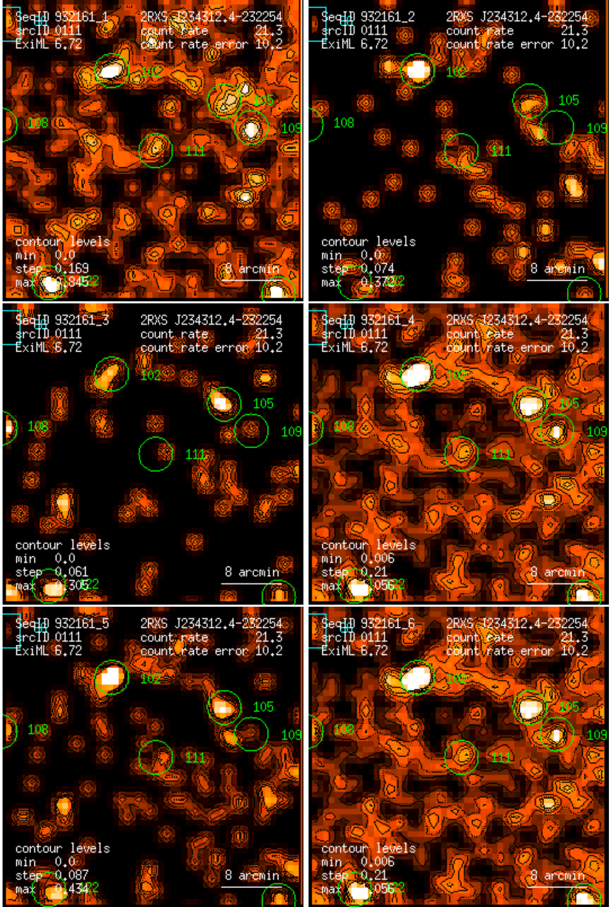
Figure 111: RASS 932161: detection 0111: band rate images, Gaussian filter: (1) PSPC channels 11 – 41, (2) 52 – 90, (3) 91 – 201, (4) 11 – 235, (5) 52 – 201, (6) 11 – 201. Broad band rates in counts/ks. Band rate contour levels in counts/ks/arcmin 2 .
