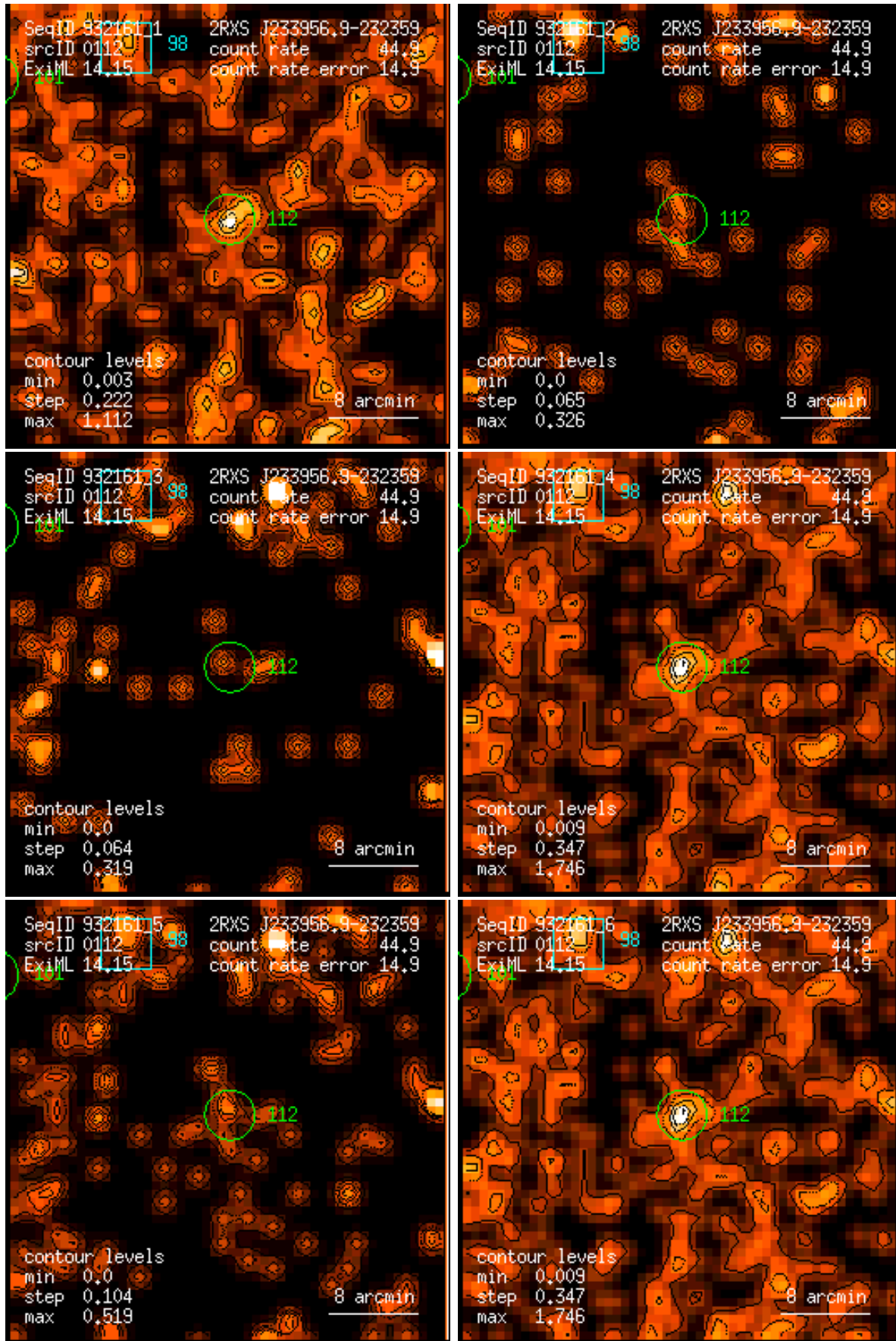
Figure 112: RASS 932161: detection 0112: band rate images, Gaussian filter: (1) PSPC channels 11 – 41, (2) 52 – 90, (3) 91 – 201, (4) 11 – 235, (5) 52 – 201, (6) 11 – 201. Broad band rates in counts/ks. Band rate contour levels in counts/ks/arcmin 2 .
