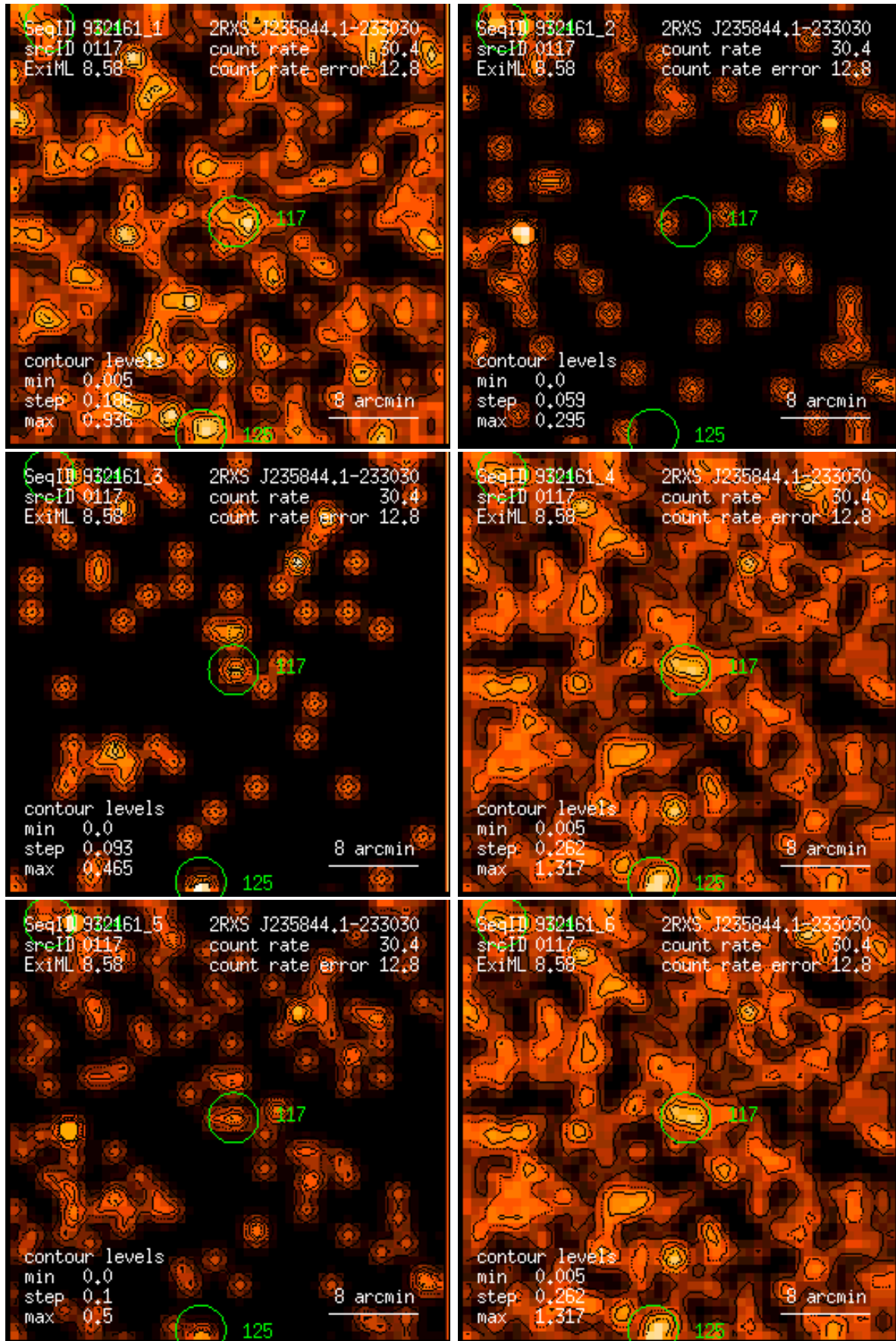
Figure 117: RASS 932161: detection 0117: band rate images, Gaussian filter: (1) PSPC channels 11 – 41, (2) 52 – 90, (3) 91 – 201, (4) 11 – 235, (5) 52 – 201, (6) 11 – 201. Broad band rates in counts/ks. Band rate contour levels in counts/ks/arcmin 2 .
