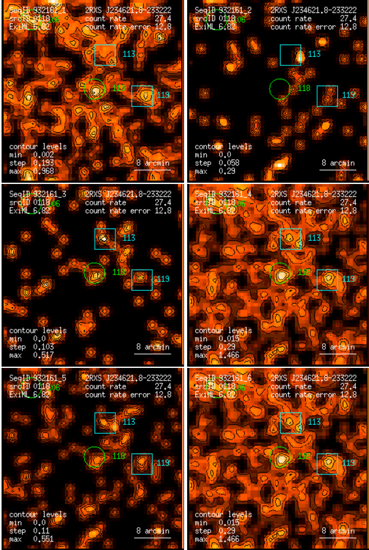
Figure 118: RASS 932161: detection 0118: band rate images, Gaussian filter: (1) PSPC channels 11 – 41, (2) 52 – 90, (3) 91 – 201, (4) 11 – 235, (5) 52 – 201, (6) 11 – 201. Broad band rates in counts/ks. Band rate contour levels in counts/ks/arcmin 2 .
