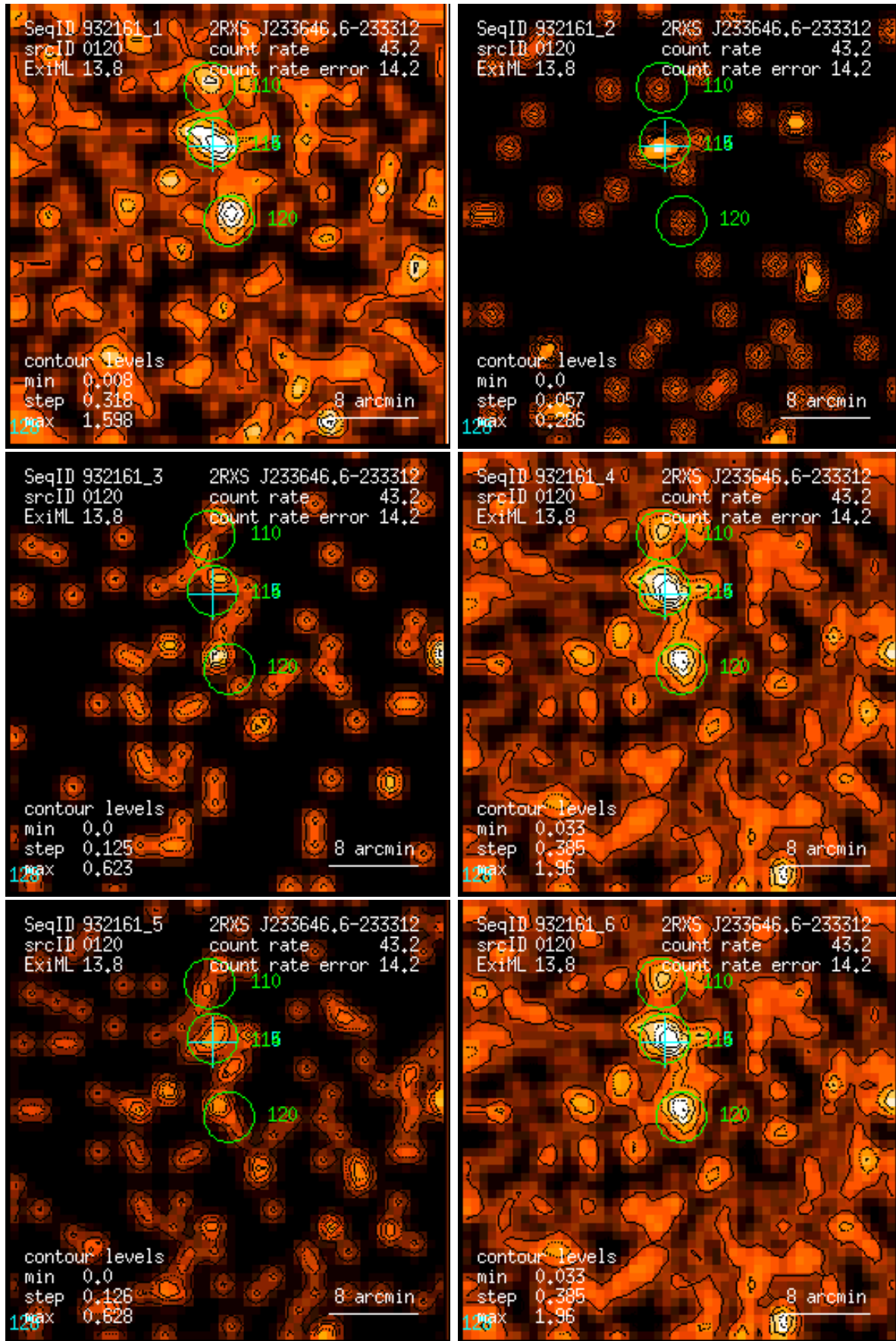
Figure 120: RASS 932161: detection 0120: band rate images, Gaussian filter: (1) PSPC channels 11 – 41, (2) 52 – 90, (3) 91 – 201, (4) 11 – 235, (5) 52 – 201, (6) 11 – 201. Broad band rates in counts/ks. Band rate contour levels in counts/ks/arcmin 2 .
