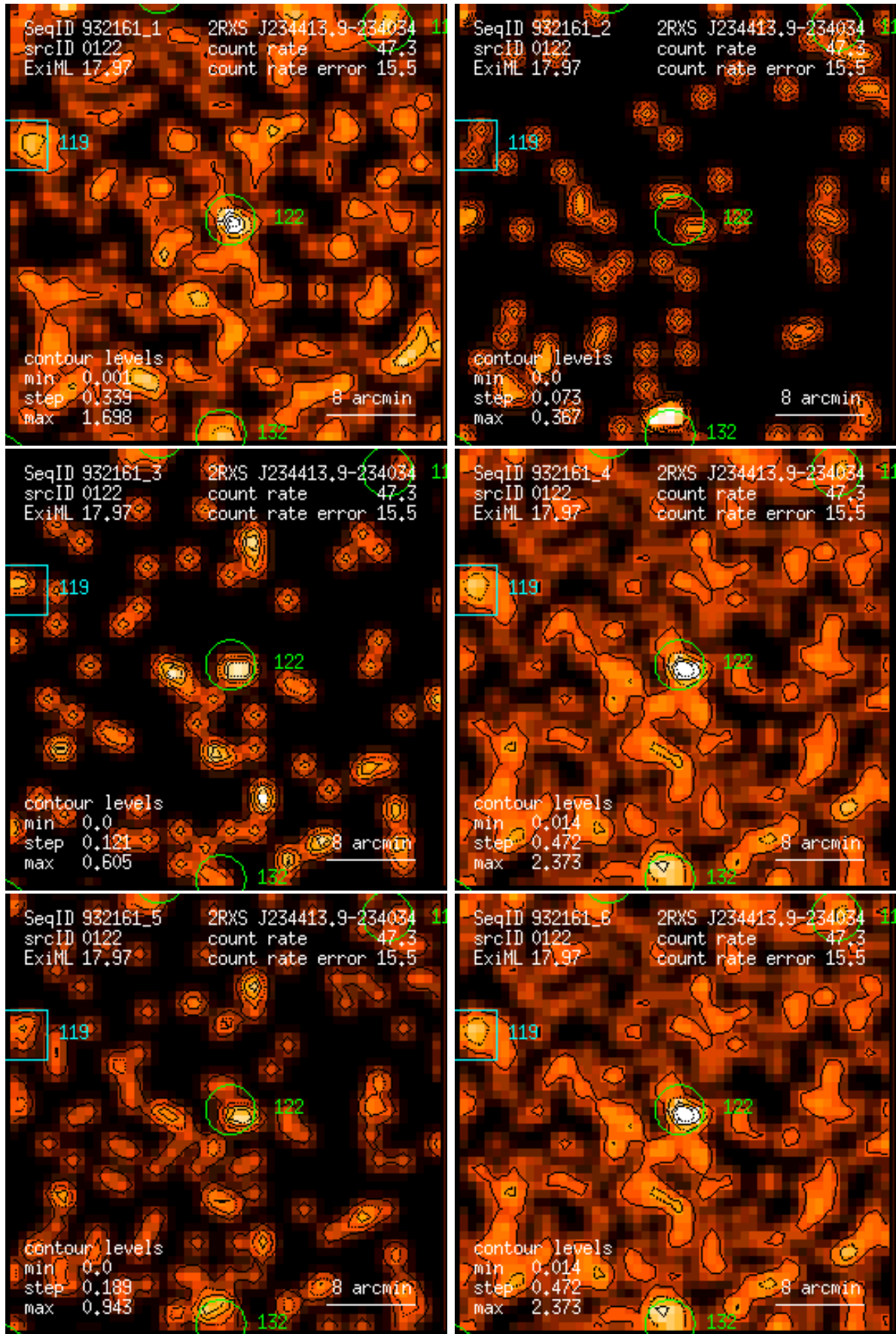
Figure 122: RASS 932161: detection 0122: band rate images, Gaussian filter: (1) PSPC channels 11 – 41, (2) 52 – 90, (3) 91 – 201, (4) 11 – 235, (5) 52 – 201, (6) 11 – 201. Broad band rates in counts/ks. Band rate contour levels in counts/ks/arcmin 2 .
