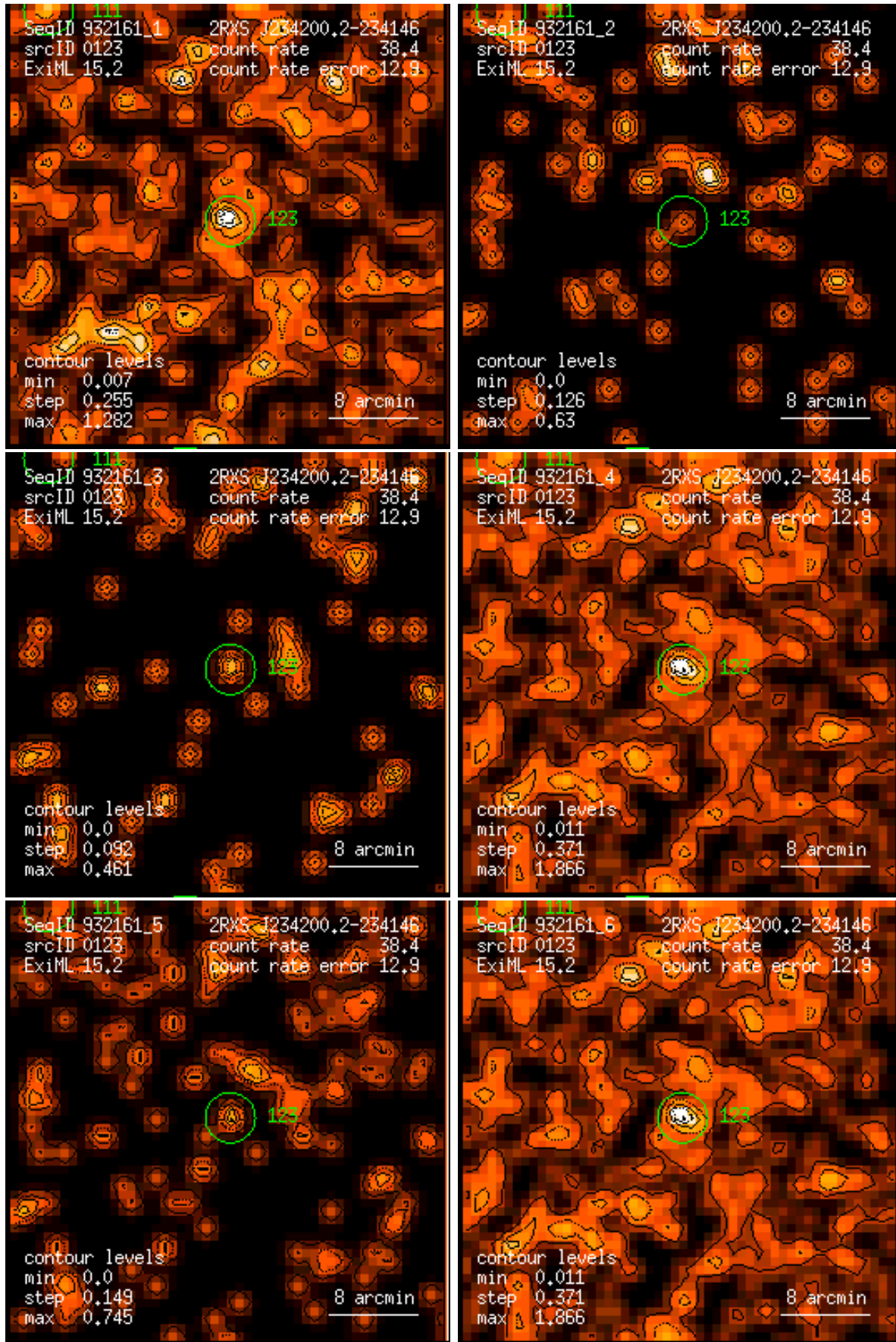
Figure 123: RASS 932161: detection 0123: band rate images, Gaussian filter: (1) PSPC channels 11 – 41, (2) 52 – 90, (3) 91 – 201, (4) 11 – 235, (5) 52 – 201, (6) 11 – 201. Broad band rates in counts/ks. Band rate contour levels in counts/ks/arcmin 2 .
