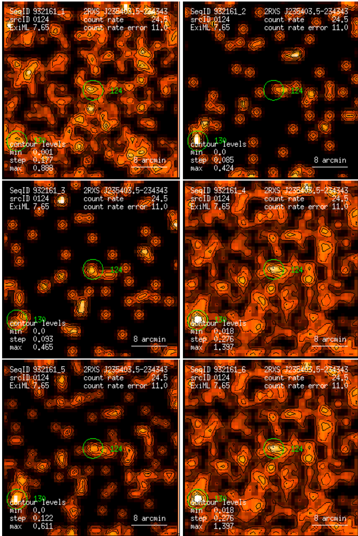
Figure 124: RASS 932161: detection 0124: band rate images, Gaussian filter: (1) PSPC channels 11 – 41, (2) 52 – 90, (3) 91 – 201, (4) 11 – 235, (5) 52 – 201, (6) 11 – 201. Broad band rates in counts/ks. Band rate contour levels in counts/ks/arcmin 2 .
