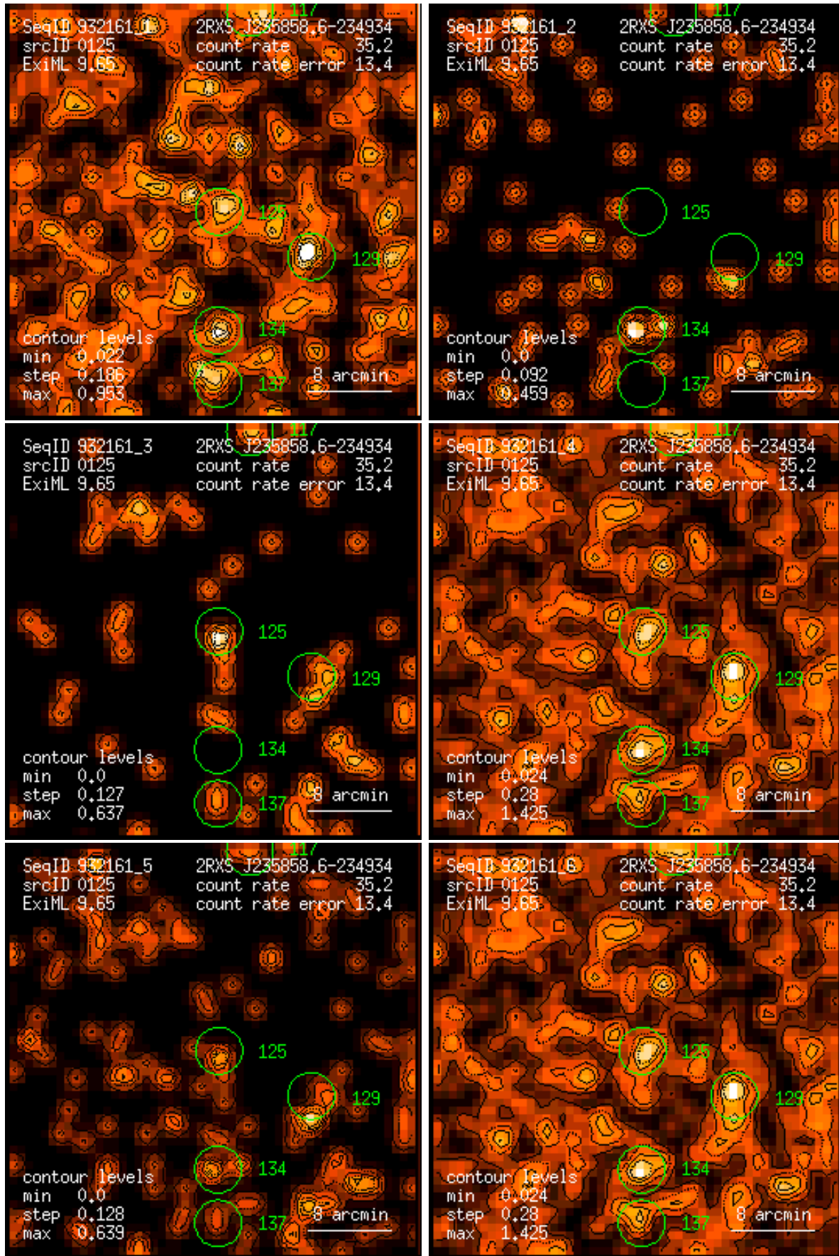
Figure 125: RASS 932161: detection 0125: band rate images, Gaussian filter: (1) PSPC channels 11 – 41, (2) 52 – 90, (3) 91 – 201, (4) 11 – 235, (5) 52 – 201, (6) 11 – 201. Broad band rates in counts/ks. Band rate contour levels in counts/ks/arcmin 2 .
