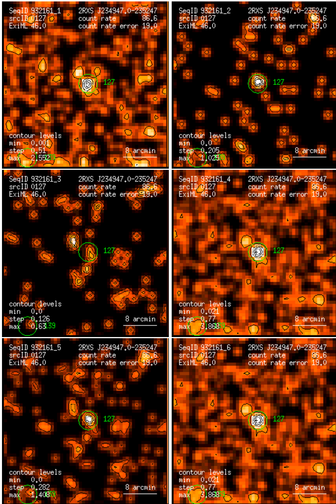
Figure 127: RASS 932161: detection 0127: band rate images, Gaussian filter: (1) PSPC channels 11 – 41, (2) 52 – 90, (3) 91 – 201, (4) 11 – 235, (5) 52 – 201, (6) 11 – 201. Broad band rates in counts/ks. Band rate contour levels in counts/ks/arcmin 2 .
