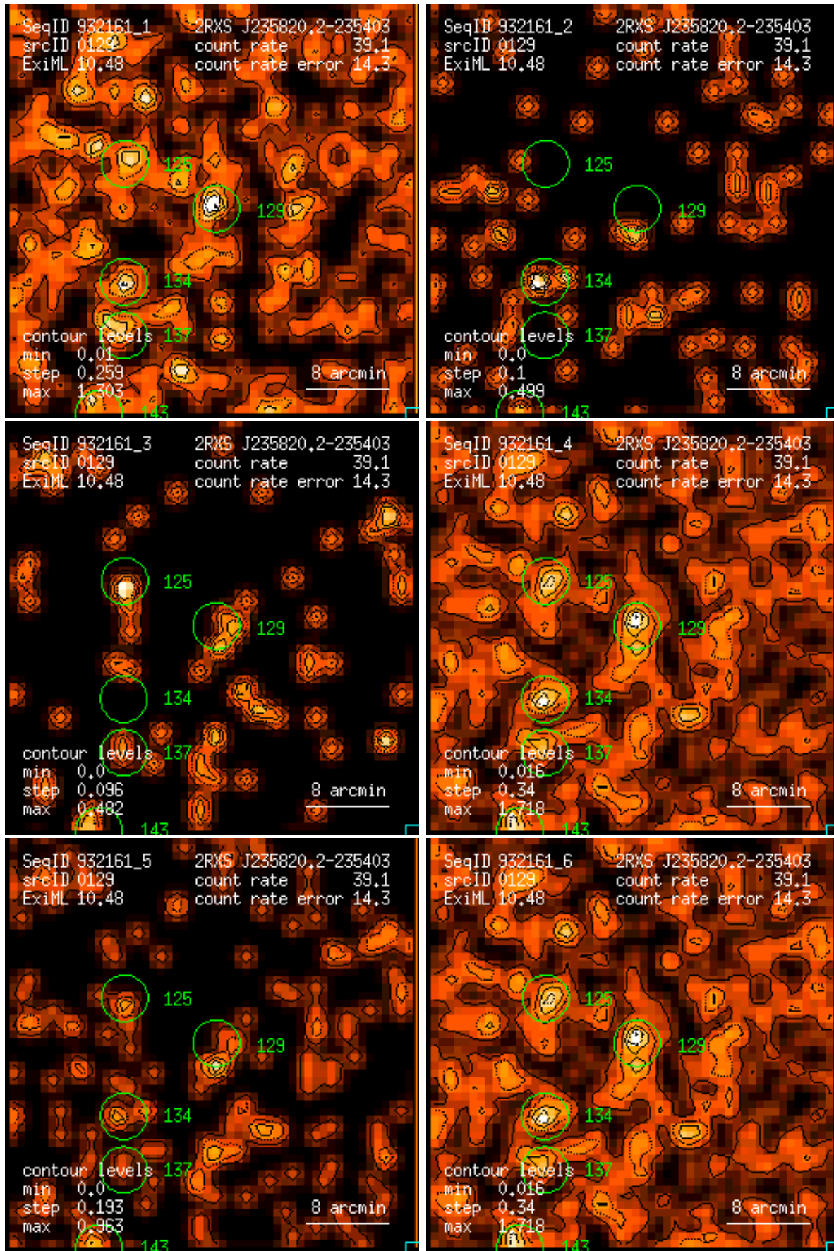
Figure 129: RASS 932161: detection 0129: band rate images, Gaussian filter: (1) PSPC channels 11 – 41, (2) 52 – 90, (3) 91 – 201, (4) 11 – 235, (5) 52 – 201, (6) 11 – 201. Broad band rates in counts/ks. Band rate contour levels in counts/ks/arcmin 2 .
