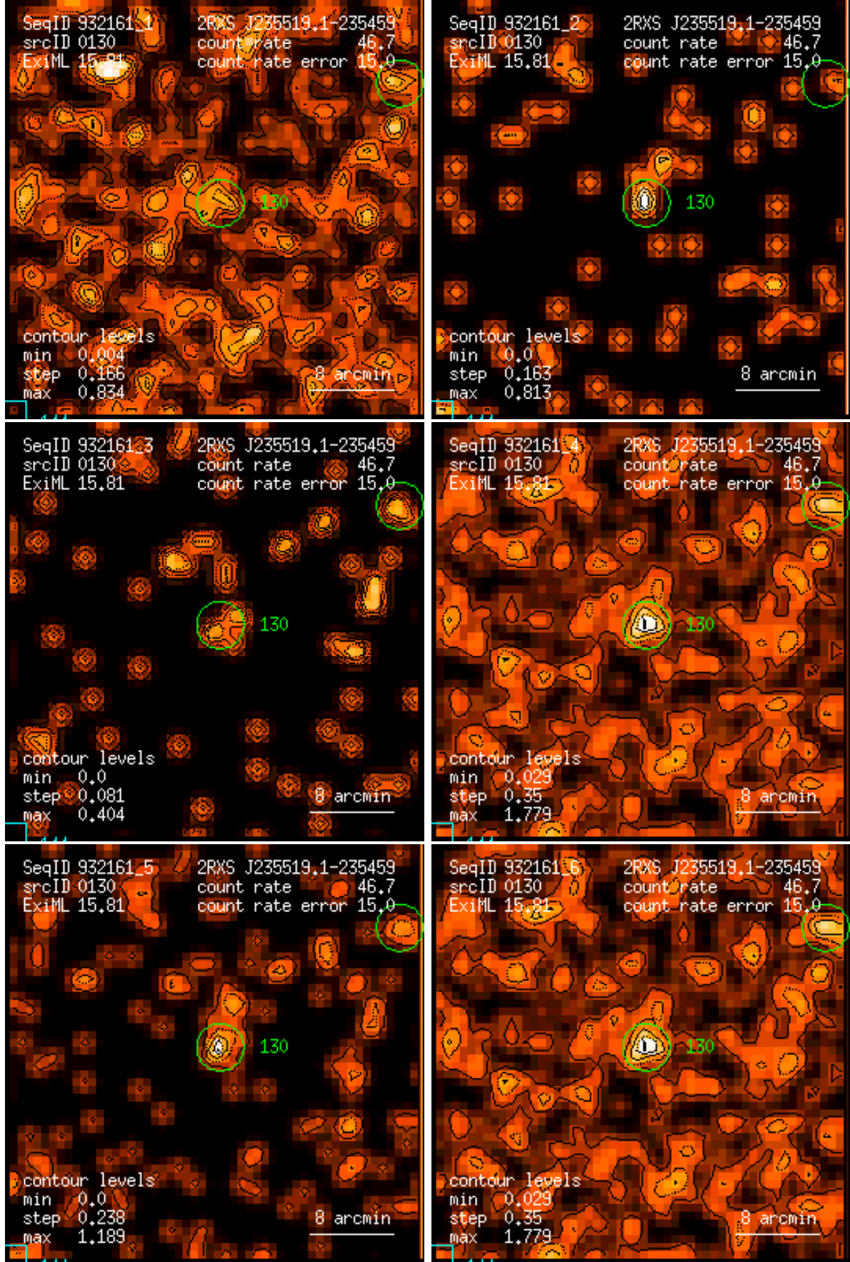
Figure 130: RASS 932161: detection 0130: band rate images, Gaussian filter: (1) PSPC channels 11 – 41, (2) 52 – 90, (3) 91 – 201, (4) 11 – 235, (5) 52 – 201, (6) 11 – 201. Broad band rates in counts/ks. Band rate contour levels in counts/ks/arcmin 2 .
