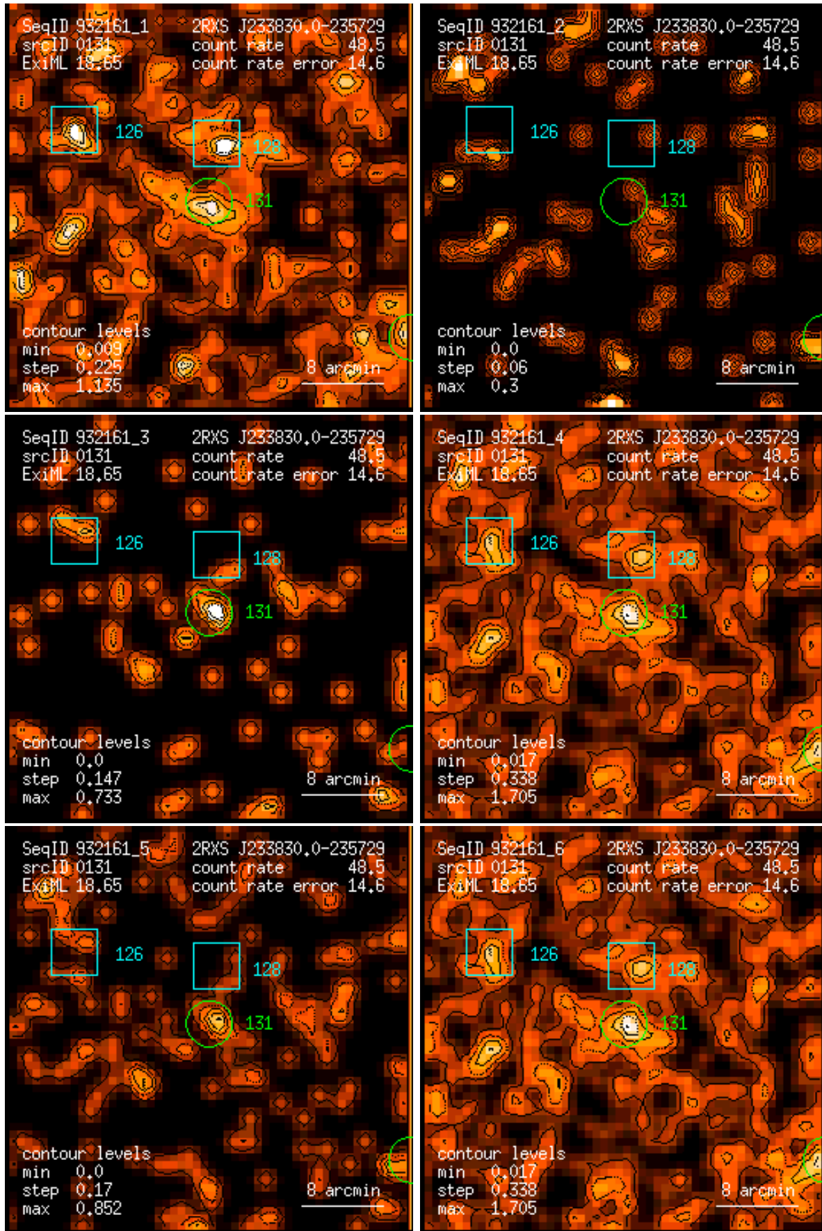
Figure 131: RASS 932161: detection 0131: band rate images, Gaussian filter: (1) PSPC channels 11 – 41, (2) 52 – 90, (3) 91 – 201, (4) 11 – 235, (5) 52 – 201, (6) 11 – 201. Broad band rates in counts/ks. Band rate contour levels in counts/ks/arcmin 2 .
