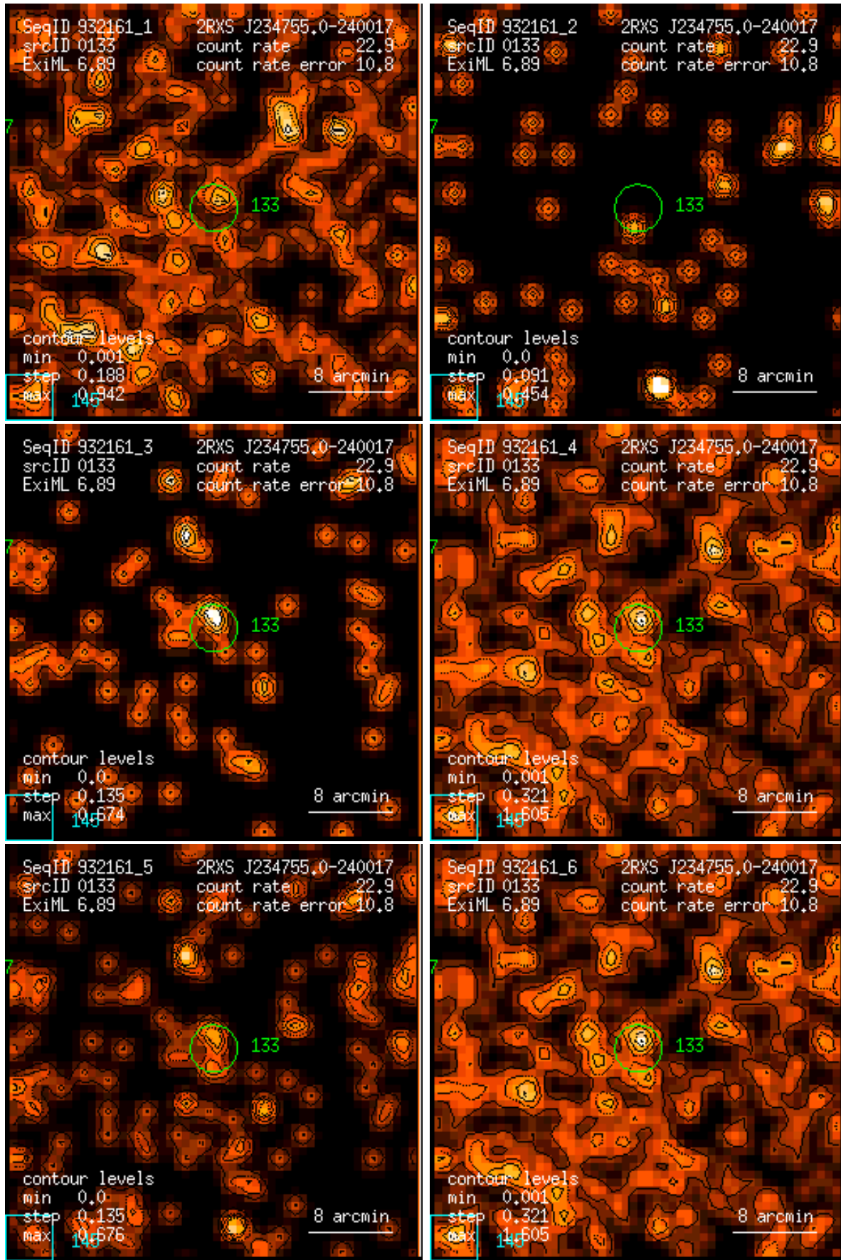
Figure 133: RASS 932161: detection 0133: band rate images, Gaussian filter: (1) PSPC channels 11 – 41, (2) 52 – 90, (3) 91 – 201, (4) 11 – 235, (5) 52 – 201, (6) 11 – 201. Broad band rates in counts/ks. Band rate contour levels in counts/ks/arcmin 2 .
