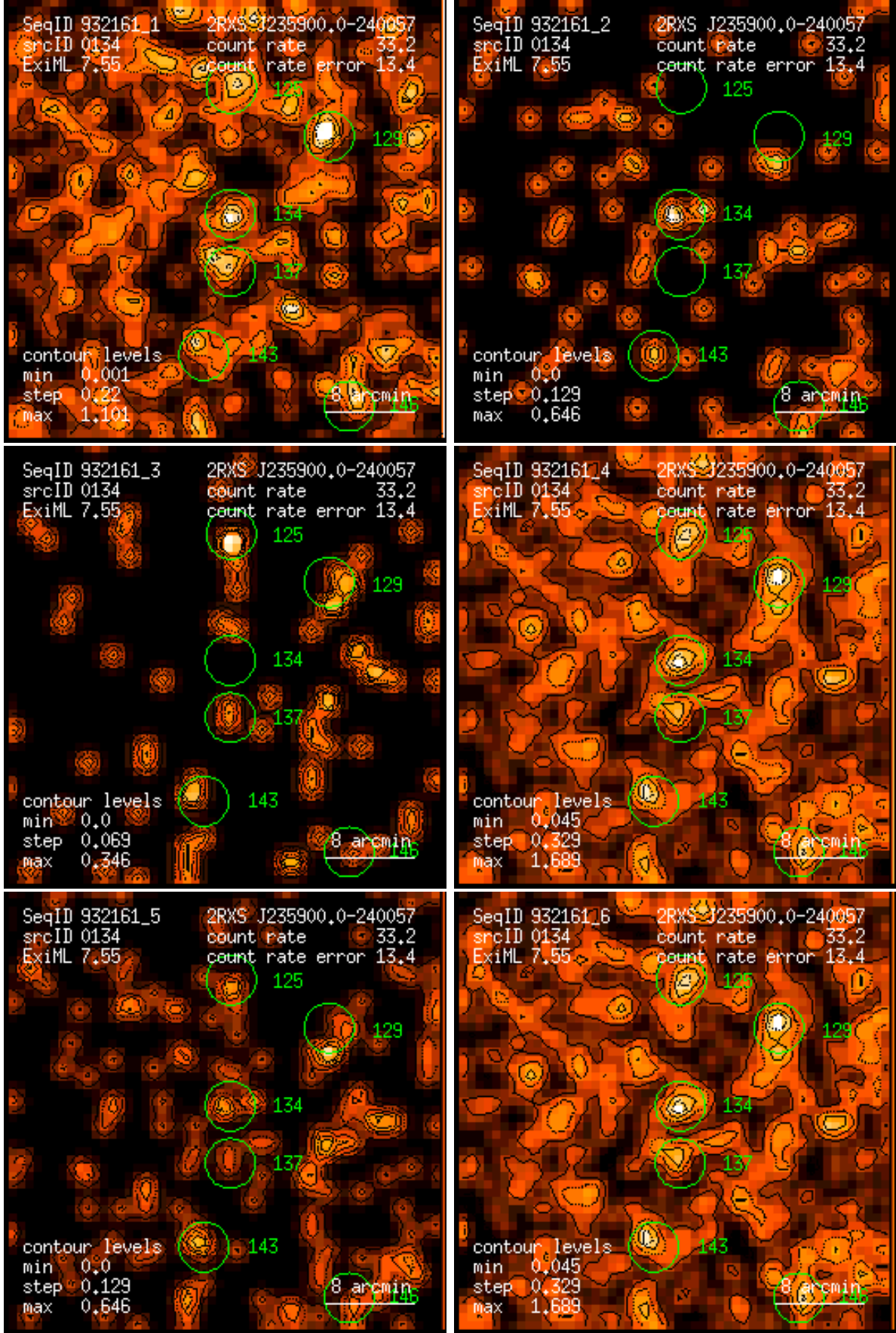
Figure 134: RASS 932161: detection 0134: band rate images, Gaussian filter: (1) PSPC channels 11 – 41, (2) 52 – 90, (3) 91 – 201, (4) 11 – 235, (5) 52 – 201, (6) 11 – 201. Broad band rates in counts/ks. Band rate contour levels in counts/ks/arcmin 2 .
