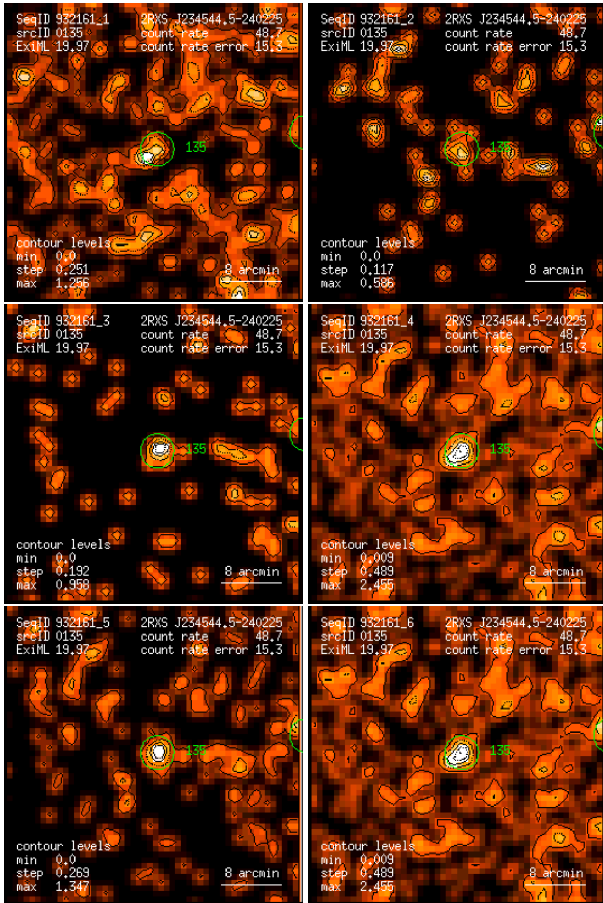
Figure 135: RASS 932161: detection 0135: band rate images, Gaussian filter: (1) PSPC channels 11 – 41, (2) 52 – 90, (3) 91 – 201, (4) 11 – 235, (5) 52 – 201, (6) 11 – 201. Broad band rates in counts/ks. Band rate contour levels in counts/ks/arcmin 2 .
