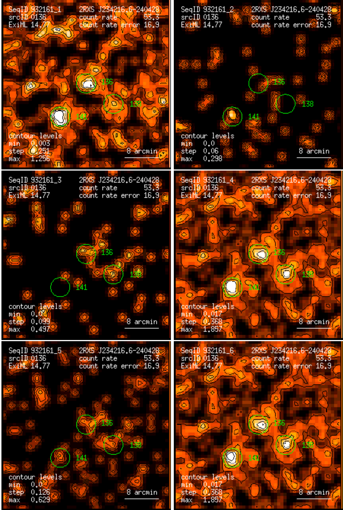
Figure 136: RASS 932161: detection 0136: band rate images, Gaussian filter: (1) PSPC channels 11 – 41, (2) 52 – 90, (3) 91 – 201, (4) 11 – 235, (5) 52 – 201, (6) 11 – 201. Broad band rates in counts/ks. Band rate contour levels in counts/ks/arcmin 2 .
