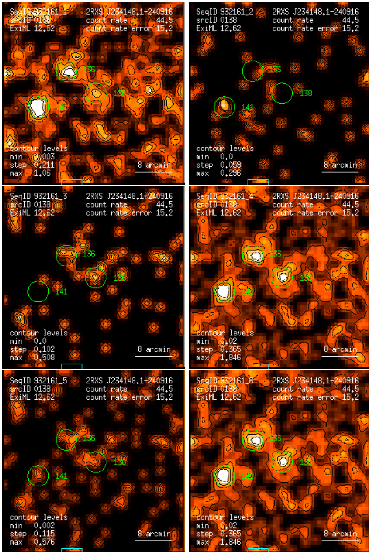
Figure 138: RASS 932161: detection 0138: band rate images, Gaussian filter: (1) PSPC channels 11 – 41, (2) 52 – 90, (3) 91 – 201, (4) 11 – 235, (5) 52 – 201, (6) 11 – 201. Broad band rates in counts/ks. Band rate contour levels in counts/ks/arcmin 2 .
