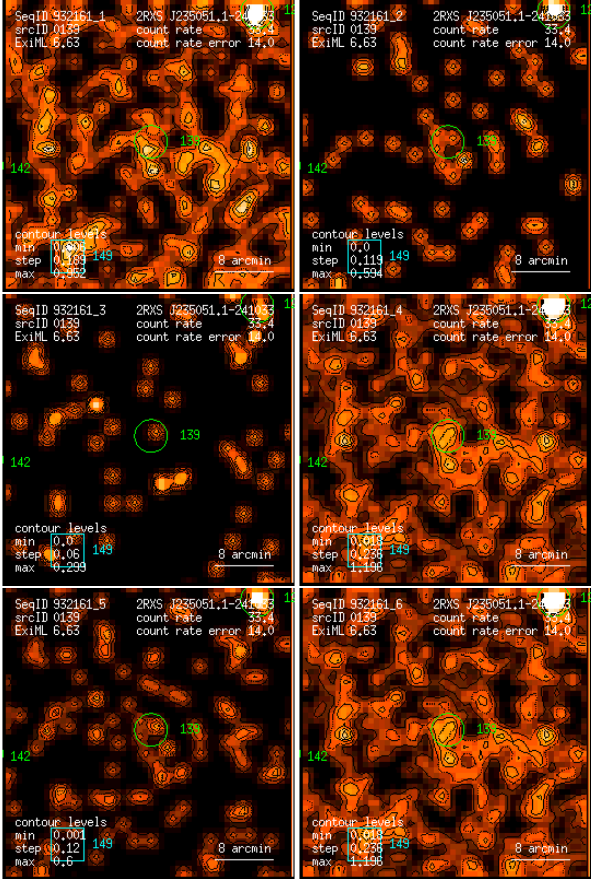
Figure 139: RASS 932161: detection 0139: band rate images, Gaussian filter: (1) PSPC channels 11 – 41, (2) 52 – 90, (3) 91 – 201, (4) 11 – 235, (5) 52 – 201, (6) 11 – 201. Broad band rates in counts/ks. Band rate contour levels in counts/ks/arcmin 2 .
