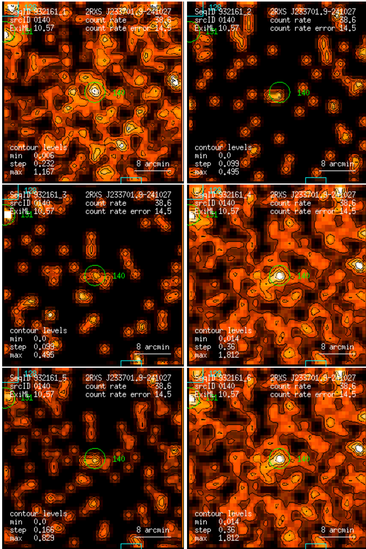
Figure 140: RASS 932161: detection 0140: band rate images, Gaussian filter: (1) PSPC channels 11 – 41, (2) 52 – 90, (3) 91 – 201, (4) 11 – 235, (5) 52 – 201, (6) 11 – 201. Broad band rates in counts/ks. Band rate contour levels in counts/ks/arcmin 2 .
